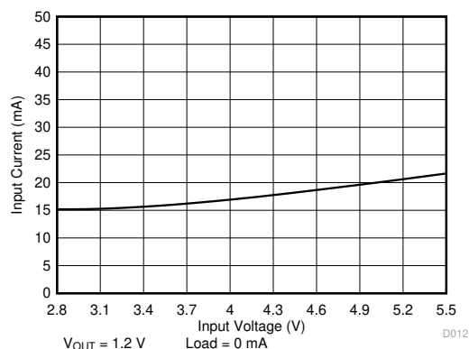
图 7-5. Active State Current Consumption vs Input Voltage, One Buck Converter Enabled in PWM Mode
