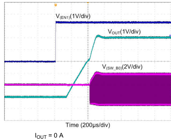
图 9-24. Boost Start-up With EN1, Forced-PWM
