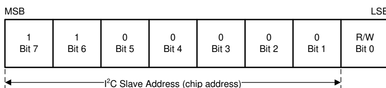
图 8-20. Device Address
