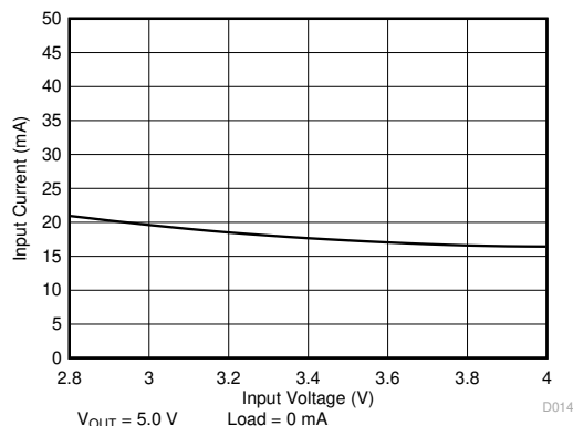
图 7-6. Active State Current Consumption vs Input Voltage, Boost Converter Enabled in PWM Mode
