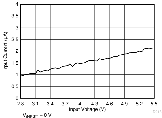
图 7-2. Shutdown Current Consumption vs Input Voltage
