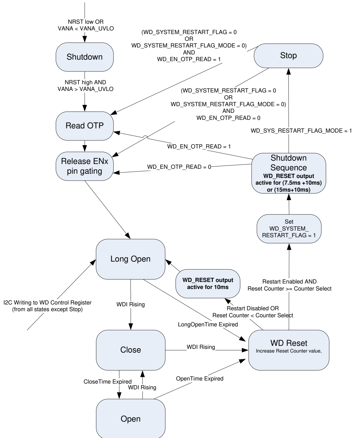
图 8-8. Watchdog Operation
