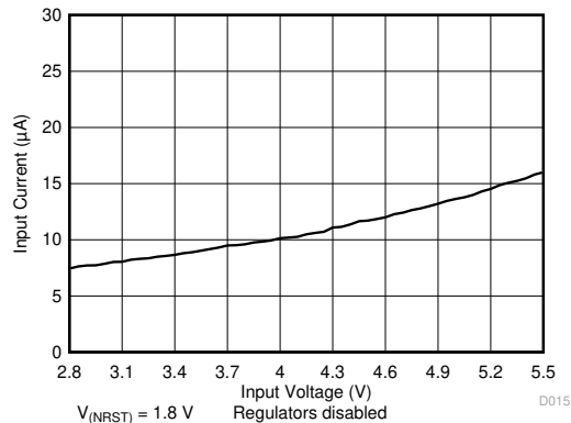
图 7-3. Standby Current Consumption vs Input Voltage
