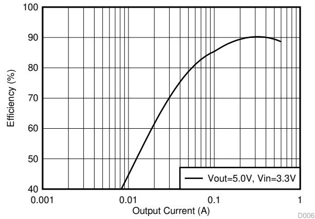
图 9-21. Boost Efficiency
