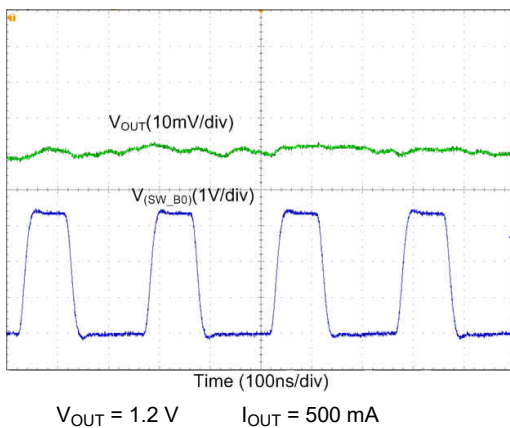
图 9-13. Buck Output Voltage Ripple, Forced-PWM Mode
