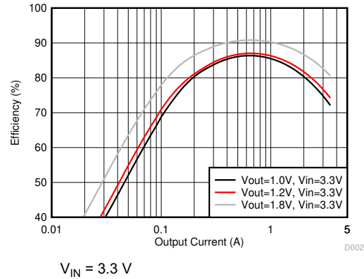
图 9-4. Buck Efficiency in Forced PWM Mode
