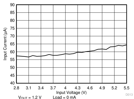
图 7-4. Active State Current Consumption vs Input Voltage, One Buck Converter Enabled in PFM Mode
