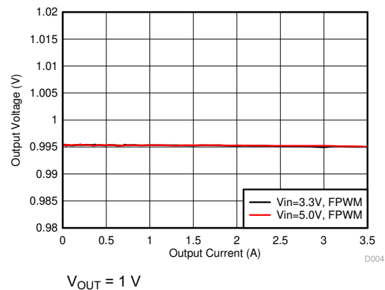
图 9-6. Buck Output Voltage vs Load Current in Forced PWM Mode
