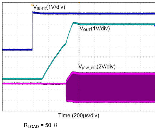
图 9-25. Boost Start-up With EN1, Forced-PWM
