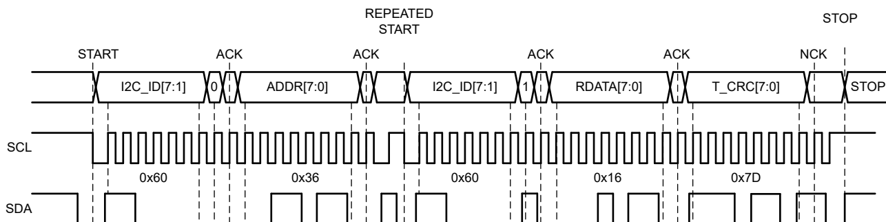
图 7-54. I 2 C Read Cycle without CRC
