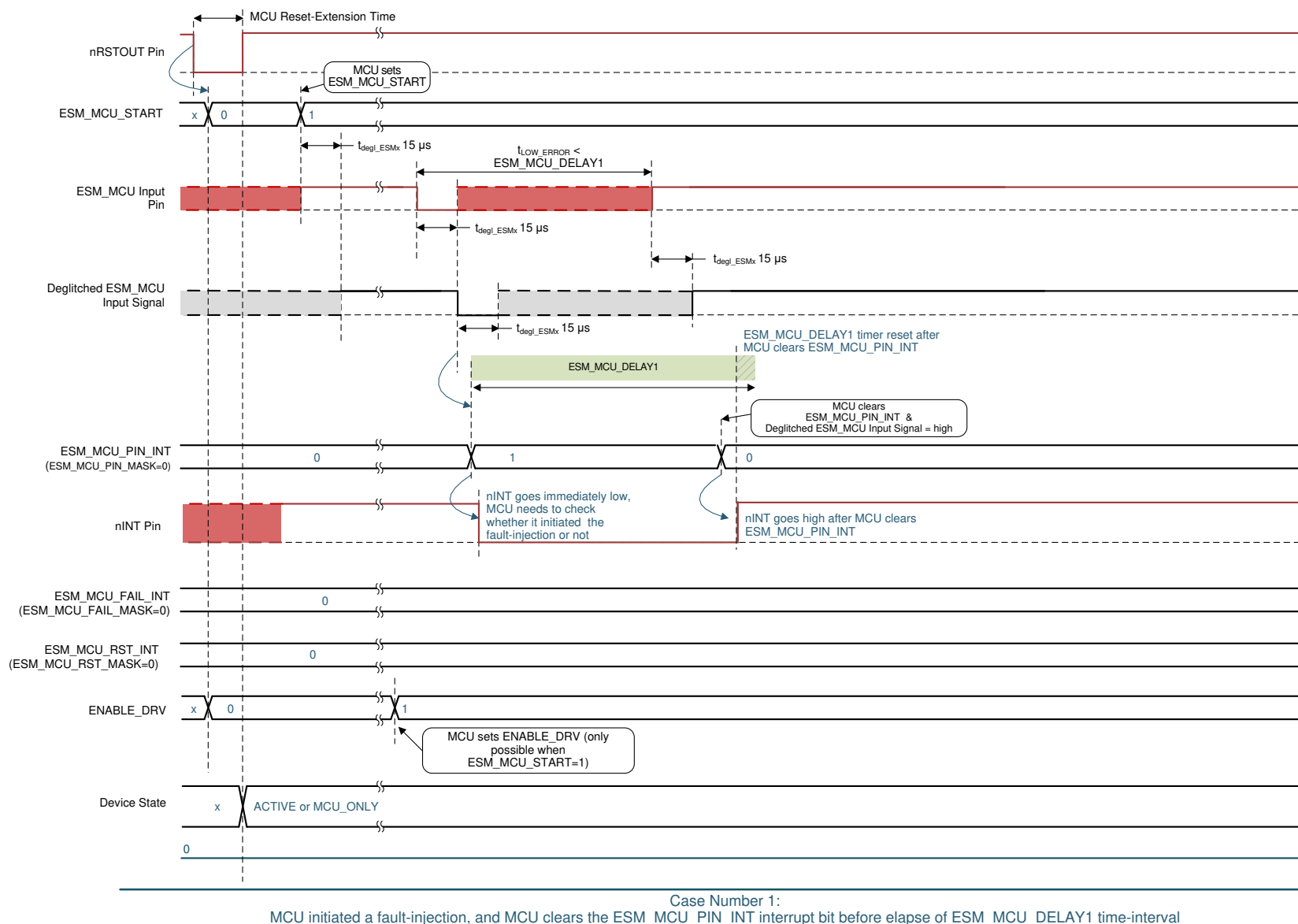
7-25. Example Waveform for ESM_MCU in Level Mode - Case Number 1: ESM_MCU Signal Recovers Before Elapse of Delay-1 time-interval
