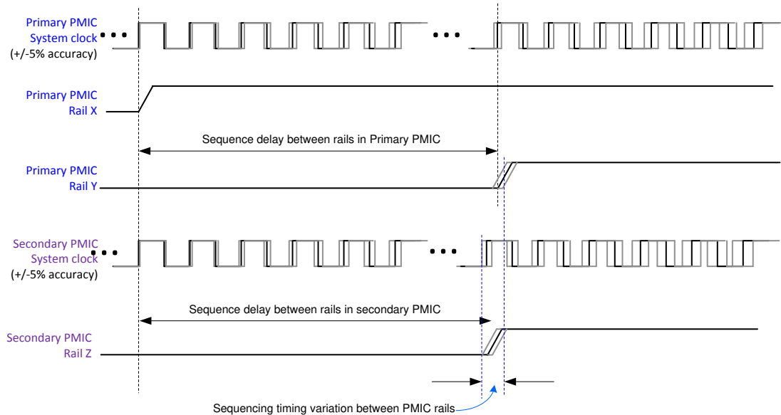
图 7-43. Multi-PMIC Rail Sequencing Timing Variation
