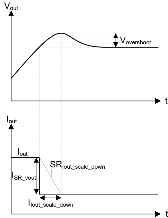
图 8-5. Overshoot
