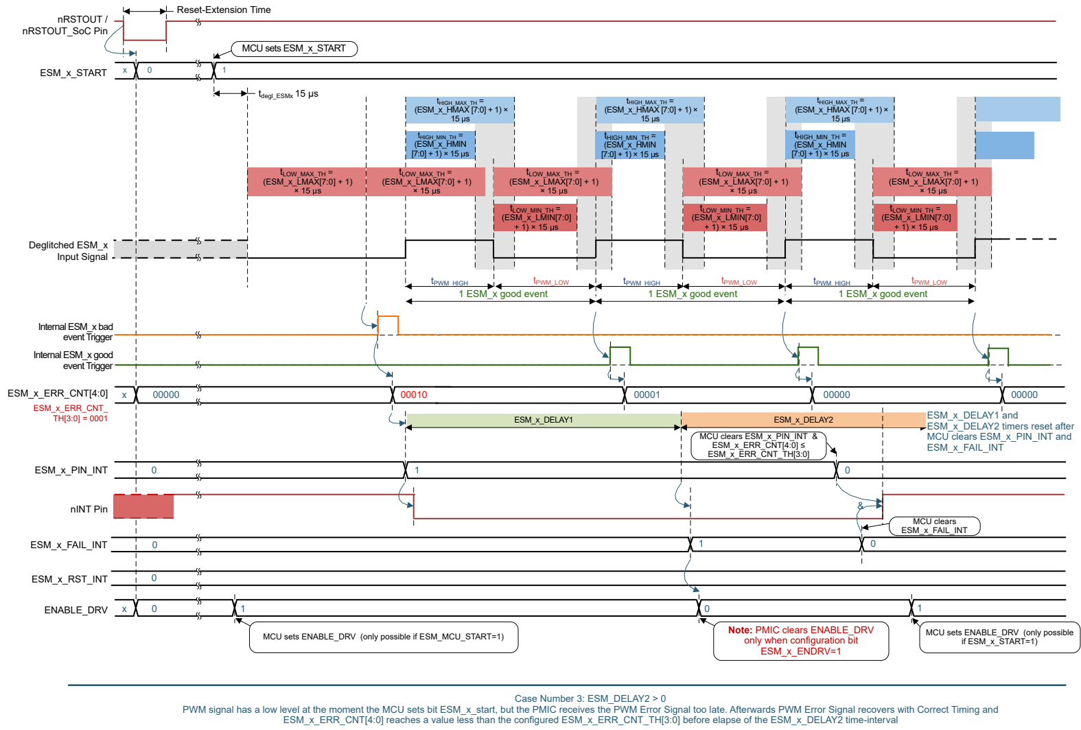
图 7-33. Example Waveform for ESM in PWM Mode – Case Number 3: ESM_MCU Starts with Low-Level at Deglitched Input Signal, but Receives Too Late a Correct PWM Signal Afterwards (The _x stand for _MCU)
