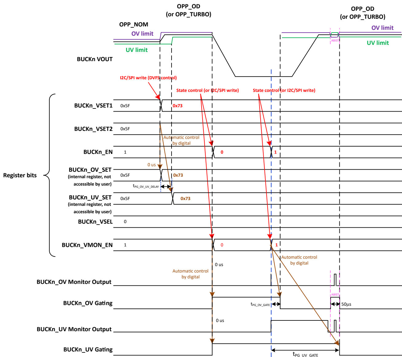
图 7-6. DVS Voltage and OV UV Threshold Level Change Timing Diagram
