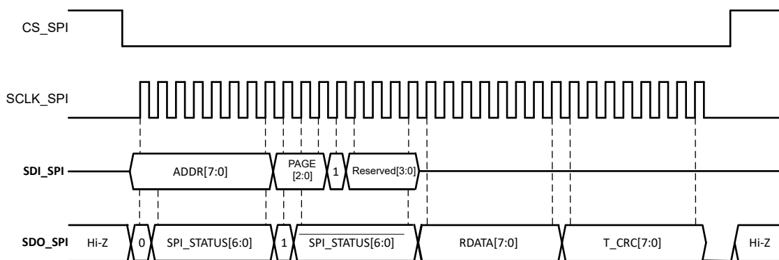
图 7-59. SPI Read Cycle with CRC
