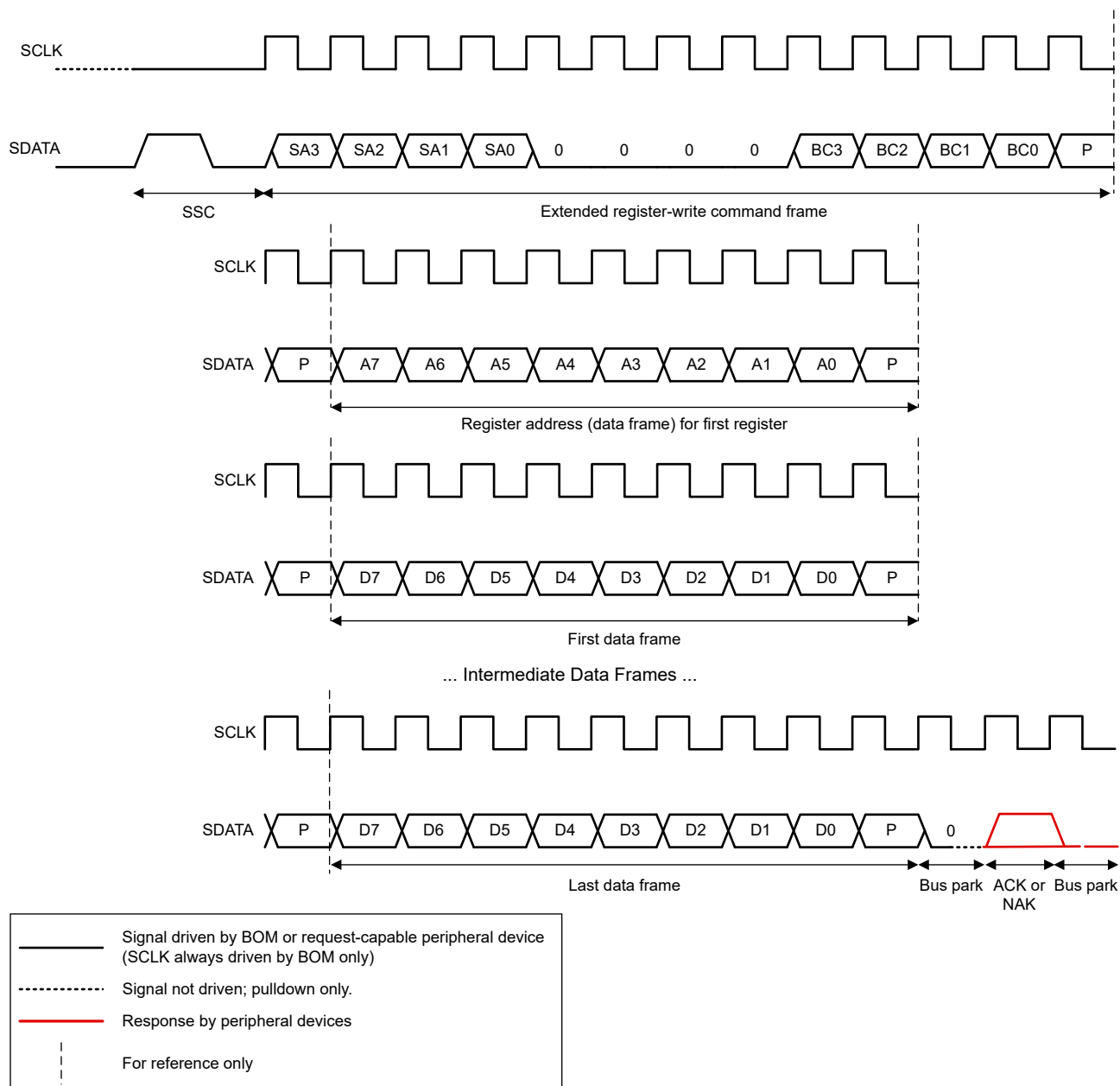
图 7-44. SPMI Extended Register Write Command
