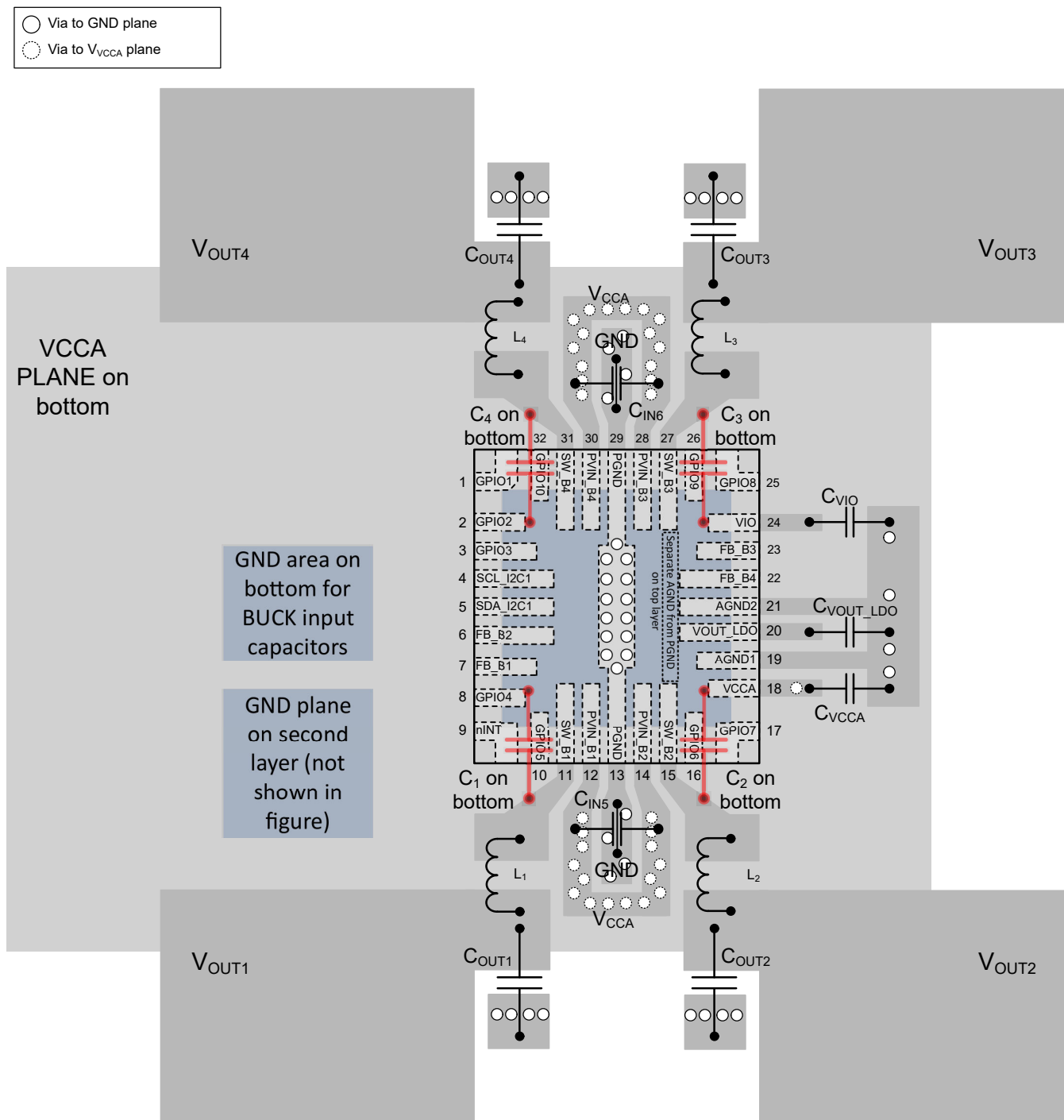
图 8-20. Device Board Layout
