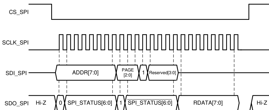
图 7-58. SPI Read Cycle
