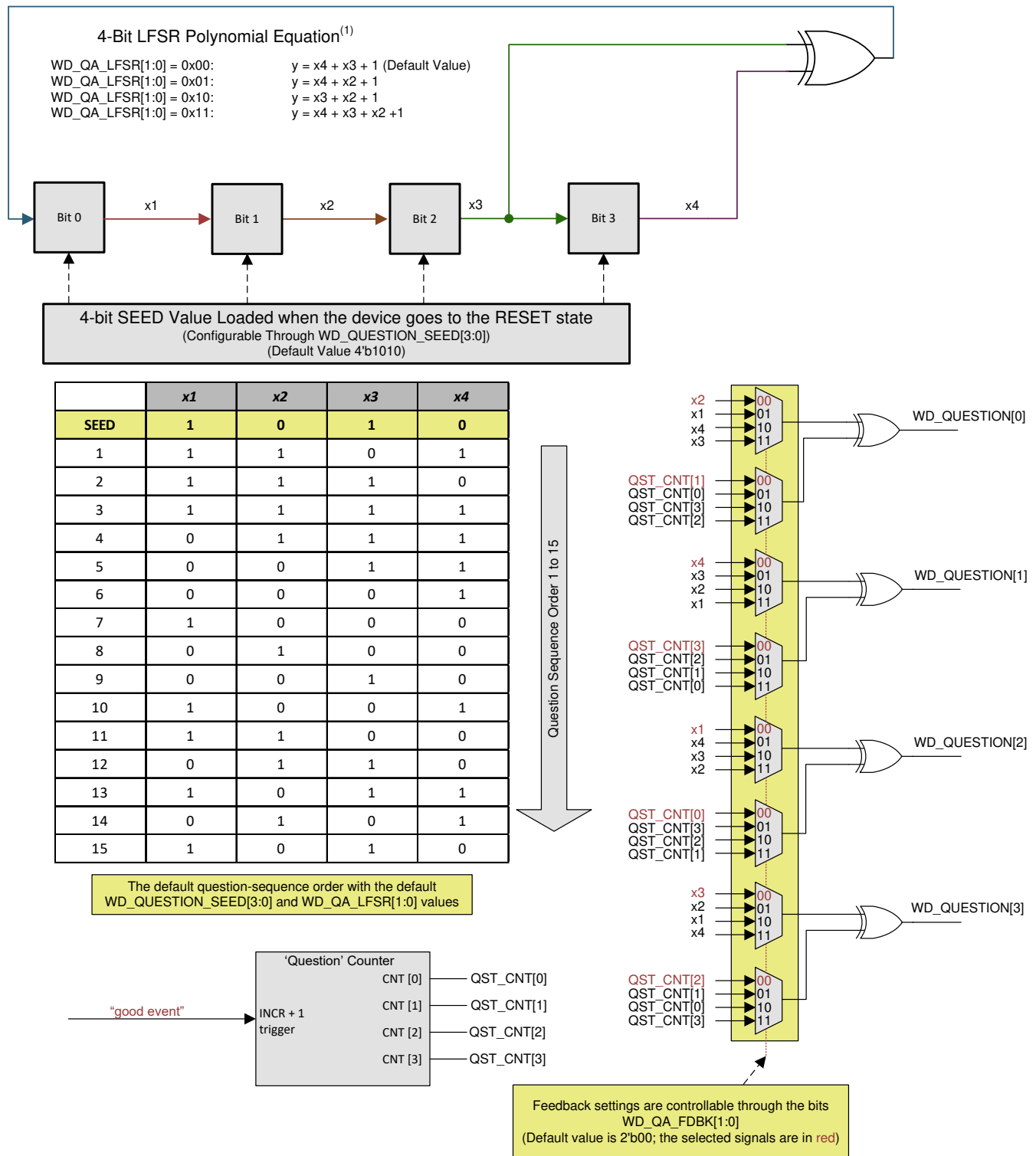
图 7-21. Watchdog Question Generation
