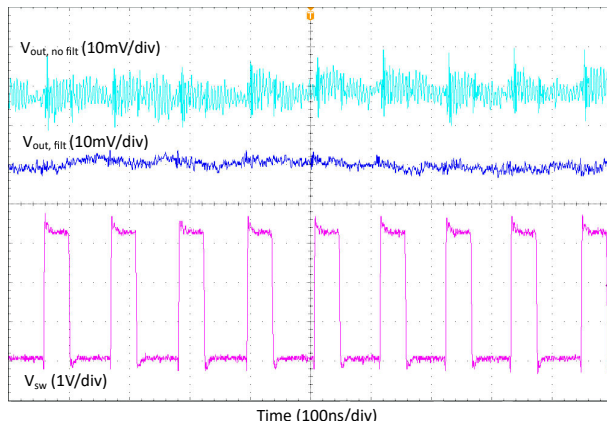
图 8-13. Output Voltage Ripple 8.8 MHz Single Phase. FPWM mode. L = 100 nH.
