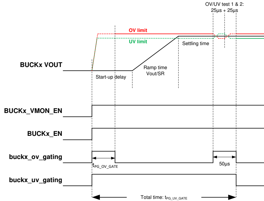
图 7-11. Timing of BUCK Regulator UV/OV Self-Test
