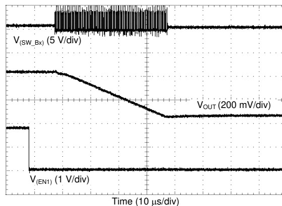
图 8-15. Shutdown with EN1
