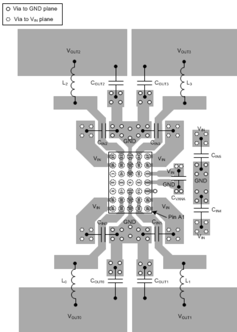
图 10-1. LP8758-EA Board Layout
