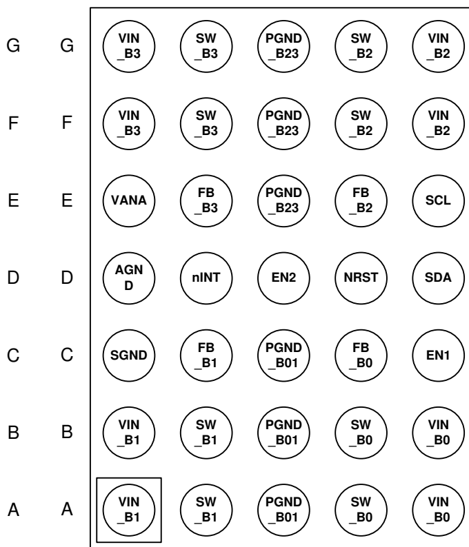
图 5-2. YFF Package 35-Pin DSBGA Bottom View
