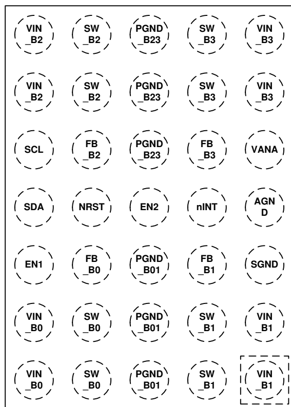
图 5-1. YFF Package 35-Pin DSBGA Top View
