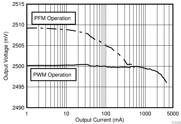
图 8-8. Output Voltage vs Load Current in PWM-PFM Mode
