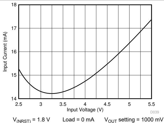
图 6-5. PWM Mode Current Consumption vs Input Voltage — One Output Enable
