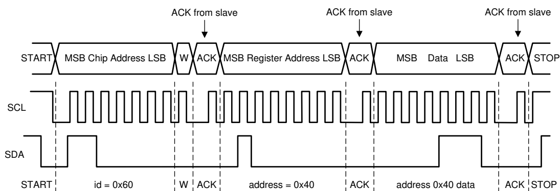
图 7-11. Write Cycle (w = write; SDA = 0), id = Device Address = 60Hex for LP8758-EA
