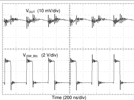
图 8-17. Output Voltage Ripple, Forced PWM Mode
