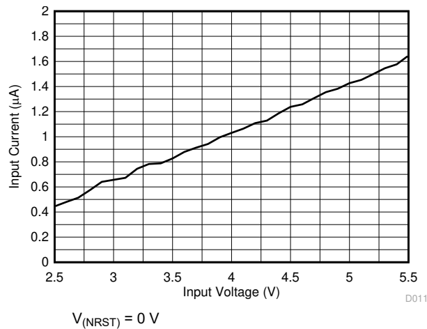
图 6-2. Shutdown Current Consumption vs Input Voltage
