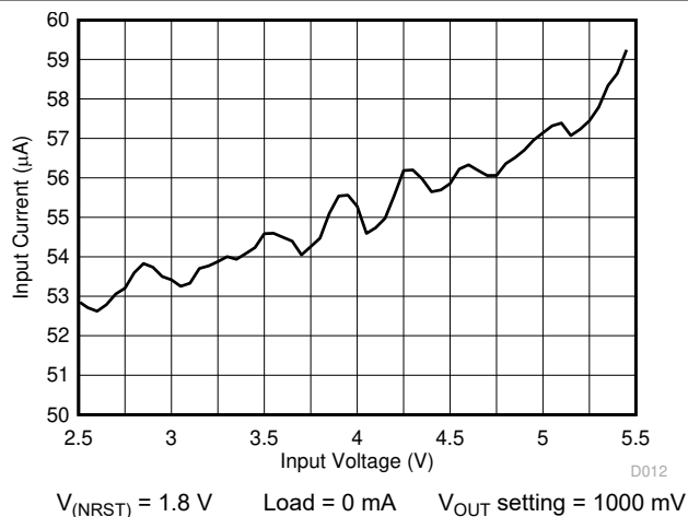
图 6-4. PFM Mode Current Consumption vs Input Voltage — One Output Enabled
