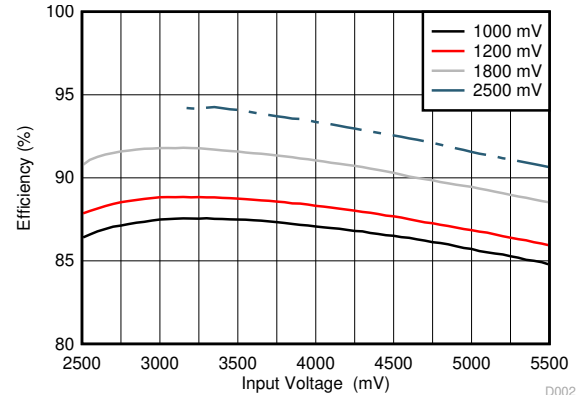
图 8-3. Efficiency vs Input Voltage in PFM Mode
