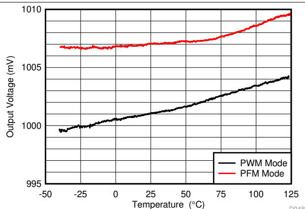
V OUT setting = 1000 mV Load = 1 A (PWM Mode) and 100 mA (PFM Mode)
