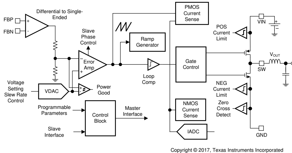
图 7-1. Detailed Block Diagram Showing One Core
