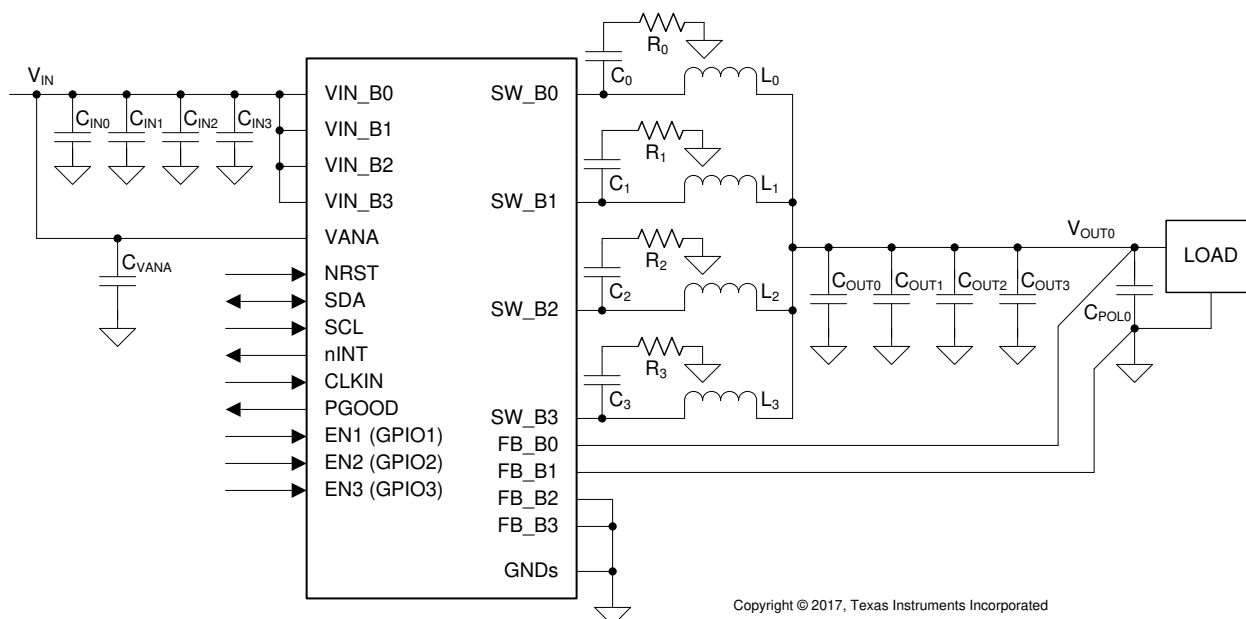
图 8-1. 4-Phase Configuration
