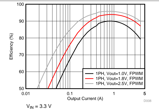
图 41. Efficiency in Forced-PWM Mode (1-Phase Output)
