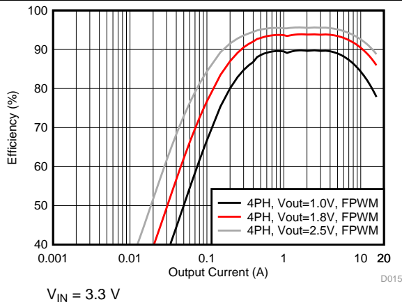
图 38. Efficiency in Forced-PWM Mode (4-Phase Output)
