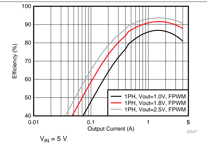
图 45. Efficiency in Forced-PWM Mode (1-Phase Output)
