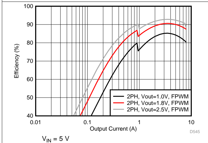
图 44. Efficiency in Forced-PWM Mode (2-Phase Output)
