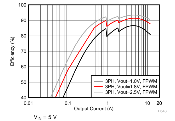
图 43. Efficiency in Forced-PWM Mode (3-Phase Output)
