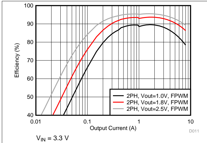
图 40. Efficiency in Forced-PWM Mode (2-Phase Output)
