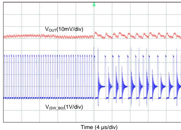
图 89. Transient from PWM-to-PFM Mode (4-Phase Output)
