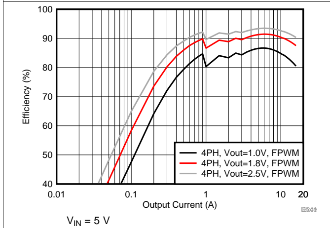
图 42. Efficiency in Forced-PWM Mode (4-Phase Output)
