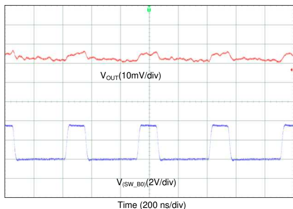
Figure 82. Output Voltage Ripple, Forced-PWM Mode (3-Phase Output)
