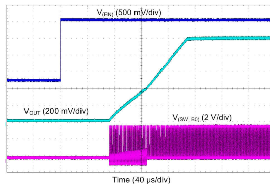
图 8-9. Buck Start-Up With EN1, Forced PWM Mode
