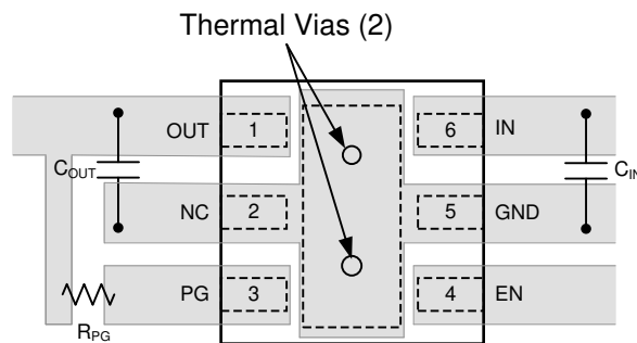
图 8-4. LP5912-EP Layout Example
