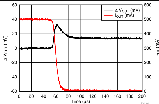
图 6-33. LP5912-0.9 Load Transient Response
