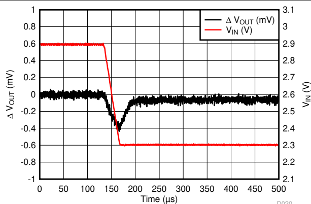
图 6-27. LP5912-0.9 Line Transient
