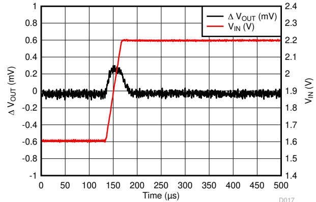
图 6-26. LP5912-0.9 Line Transient
