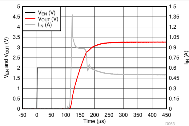
图 6-52. LP5912-3.3 Inrush Current
