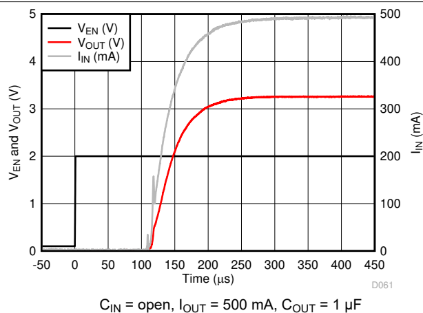
图 6-50. LP5912-3.3 Inrush Current
