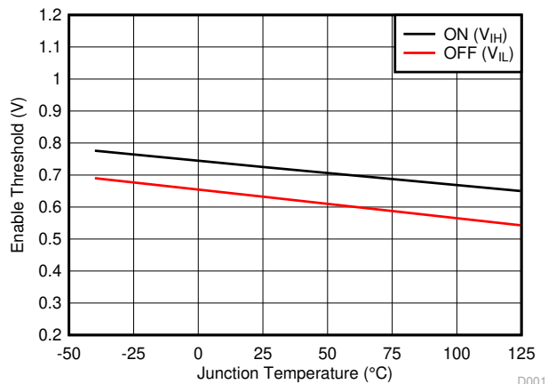
图 6-1. V_{EN} Threshold vs Temperature
