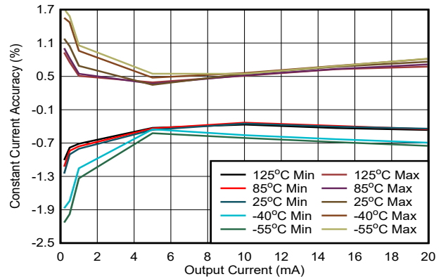
图 7-5. Channel to Channel Accuracy vs Output Current
