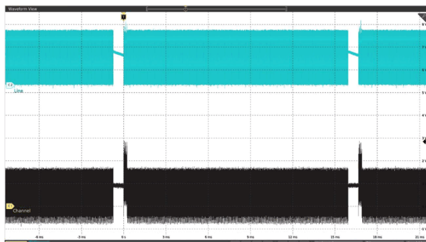
图 9-7. Line and Channel Waveform in One Frame (GSn = 0x0001h)
