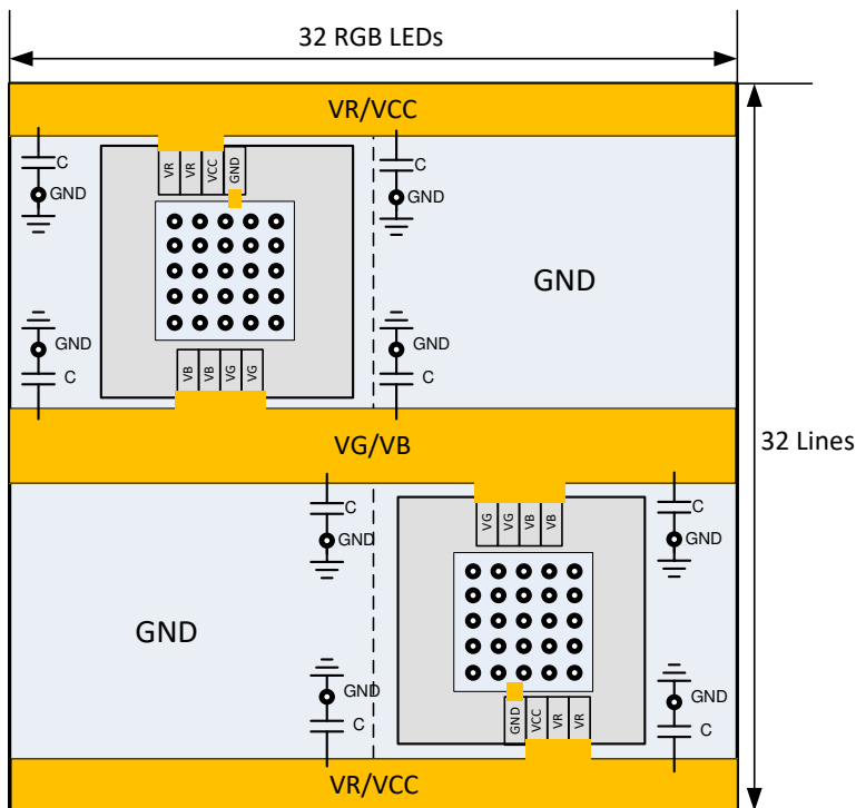
图 9-9. Power Rails Routing Suggestion
