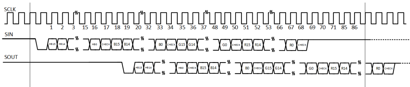
图 8-22. Data Write Command with Broadcast (Timing Diagram)
