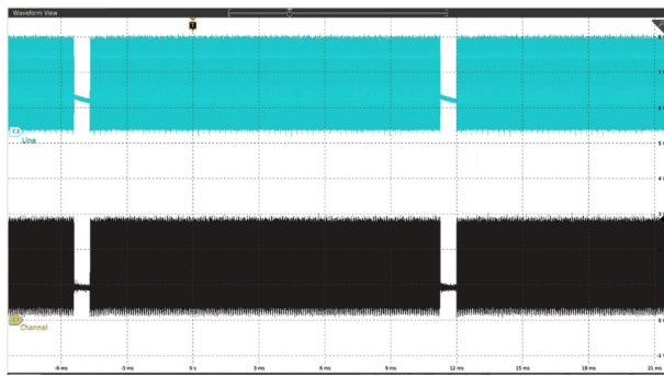
图 9-5. Line and Channel Waveform in One Frame (GSn = 0xFFFFh)
