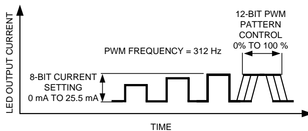
Figure 16. LED Pattern and Current Control Principle
