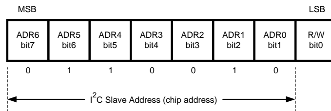
Figure 20. LP5523 Chip Address
