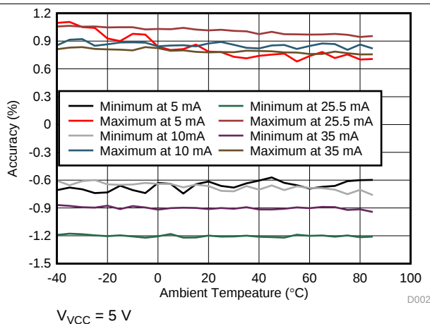
图 6. Channel-to-Channel Accuracy
