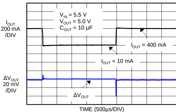
Figure 34. Load Transient
