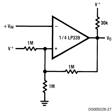
Inverting Comparator with Hysteresis
