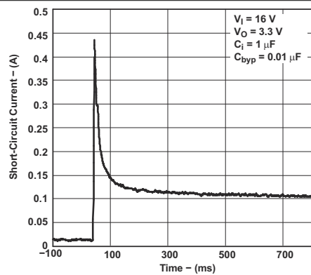
图 6-9. Short-Circuit Current vs Time for Legacy Chip
