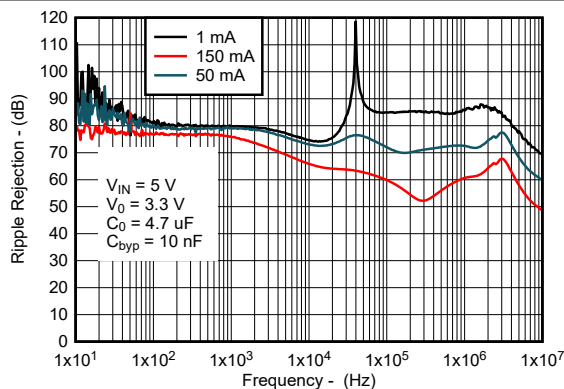
图 6-21. Ripple Rejection vs Frequency for New Chip
