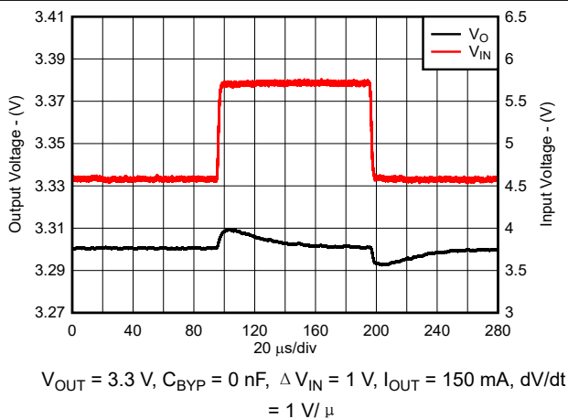
图 8-10. Line Transient Response for New Chip
