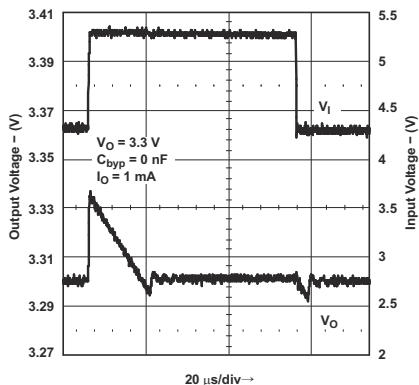
图 8-13. Line Transient Response for Legacy Chip
