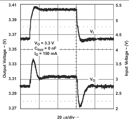
图 8-9. Line Transient Response for Legacy Chip
