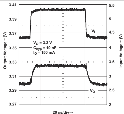
图 8-11. Line Transient Response for Legacy Chip
