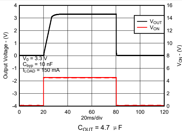
图 8-24. Turn-On Time for New Chip
