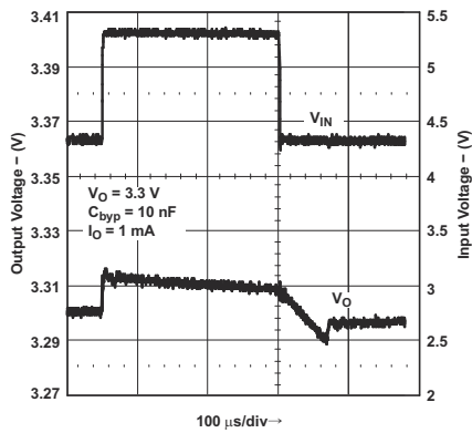
图 8-15. Line Transient Response for Legacy Chip
