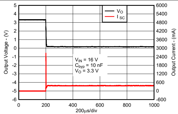
图 6-10. Short-Circuit Current vs Time for New Chip
