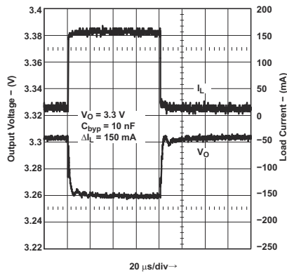
图 8-3. Load Transient Response for Legacy Chip
