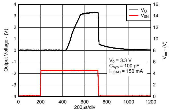
图 8-18. Turn-On Time for New Chip
