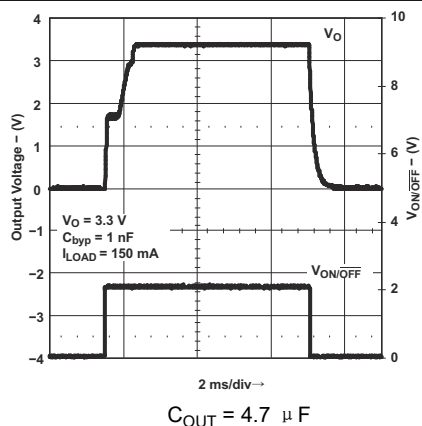
图 8-21. Turn-On Time for Legacy Chip
