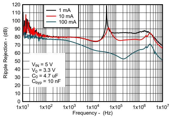
图 6-25. Ripple Rejection vs Frequency for New Chip
