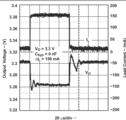
图 8-5. Load Transient Response for Legacy Chip
