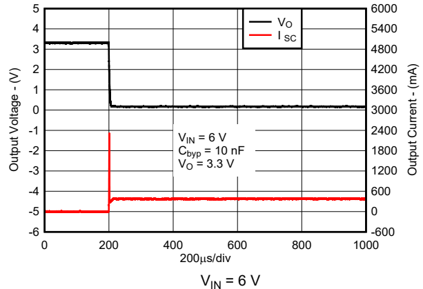
图 6-10. Short-Circuit Current vs Time for New Chip
