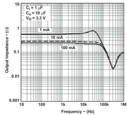
图 6-26. Output Impedance vs Frequency for Legacy Chip
