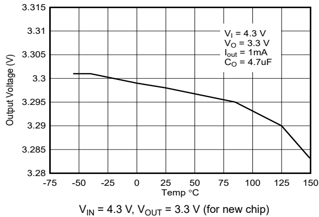
图 6-3. Output Voltage vs Temperature for New Chip
