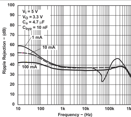
图 6-22. Ripple Rejection vs Frequency for Legacy Chip
