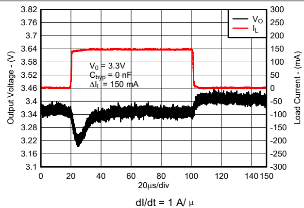
图 8-8. Load Transient Response for New Chip
