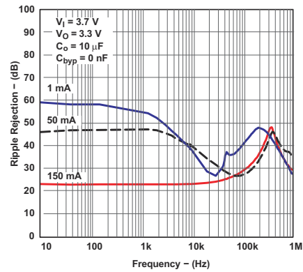
图 5-20. Ripple Rejection vs Frequency for Legacy Chip
