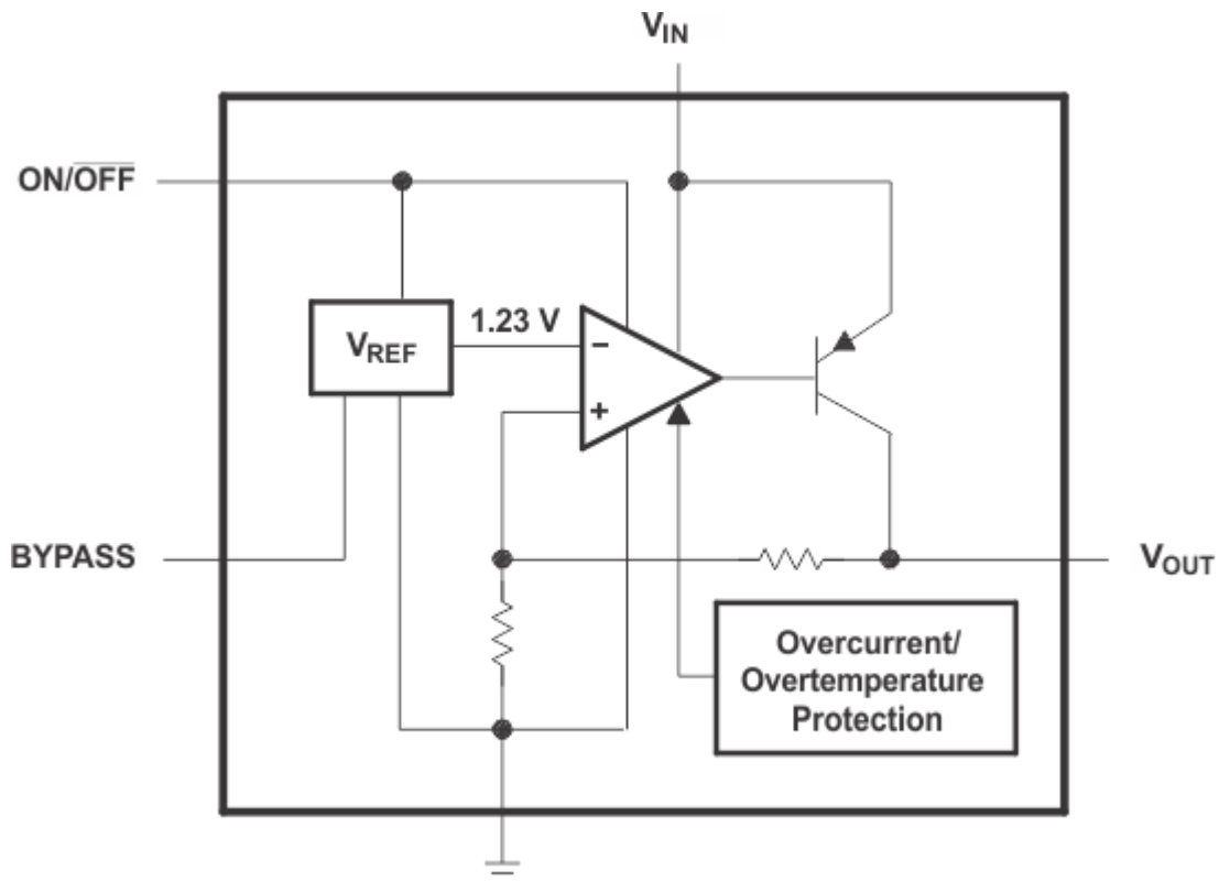
图 6-1. Functional Block Diagram (Legacy Chip)
