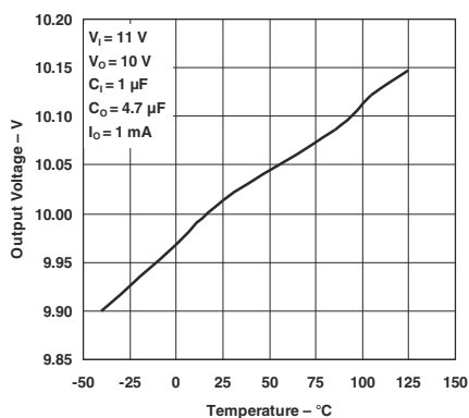
图 5-1. Output Voltage vs Temperature for Legacy Chip
