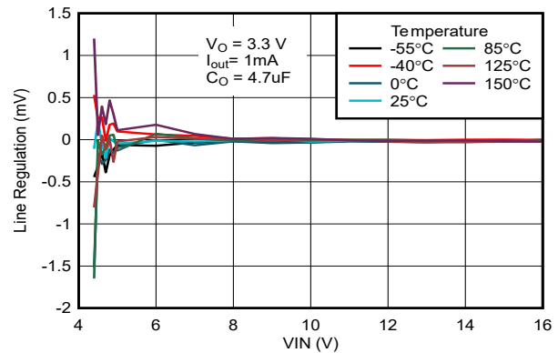
图 5-8. Output Regulation vs Input Voltage for New Chip
