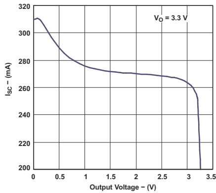
图 5-13. Short-Circuit Current vs Output Voltage for Legacy Chip
