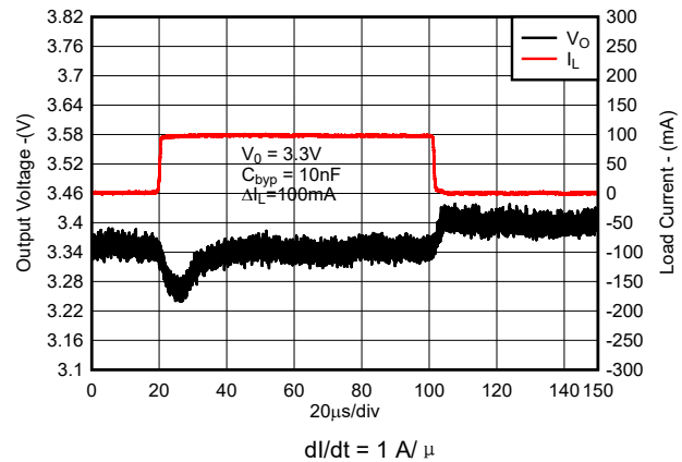
图 7-4. Load Transient Response for New Chip
