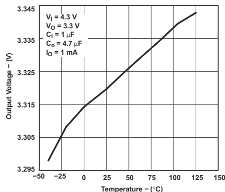
图 5-2. Output Voltage vs Temperature for Legacy Chip
