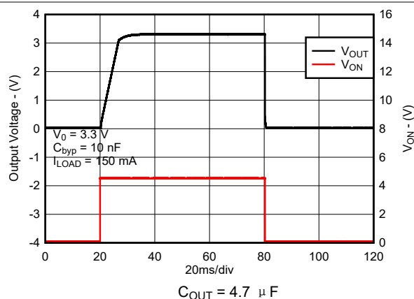
图 7-24. Turn-On Time for New Chip
