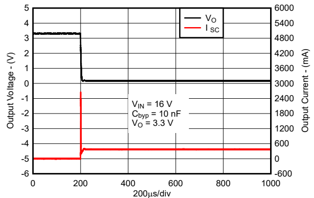
图 5-10. Short-Circuit Current vs Time for New Chip
