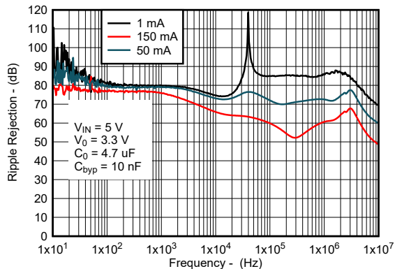
图 5-21. Ripple Rejection vs Frequency for New Chip
