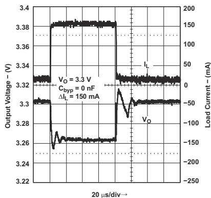
图 7-5. Load Transient Response for Legacy Chip
