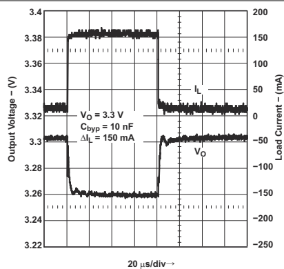
图 7-3. Load Transient Response for Legacy Chip
