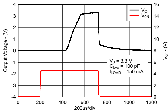
图 7-18. Turn-On Time for New Chip
