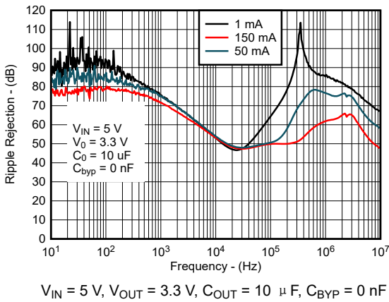
图 5-19. Ripple Rejection vs Frequency for New Chip
