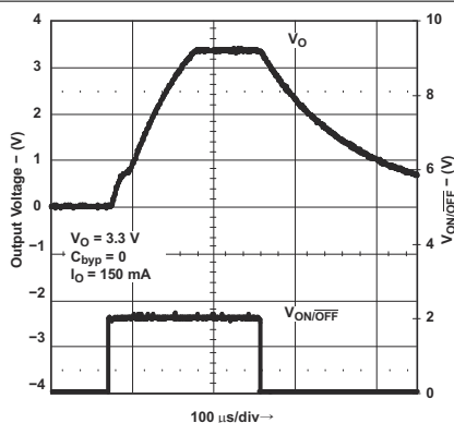
图 7-17. Turn-On Time for Legacy Chip
