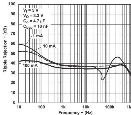
图 5-22. Ripple Rejection vs Frequency for Legacy Chip
