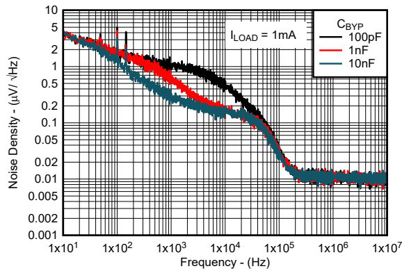
图 5-31. Output Noise Density vs Frequency for New Chip
