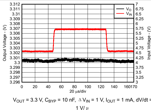
图 7-16. Line Transient Response for New Chip
