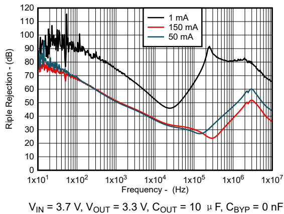
图 5-21. Ripple Rejection vs Frequency for New Chip
