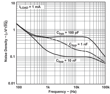
图 5-28. Output Noise Density vs Frequency for Legacy Chip
