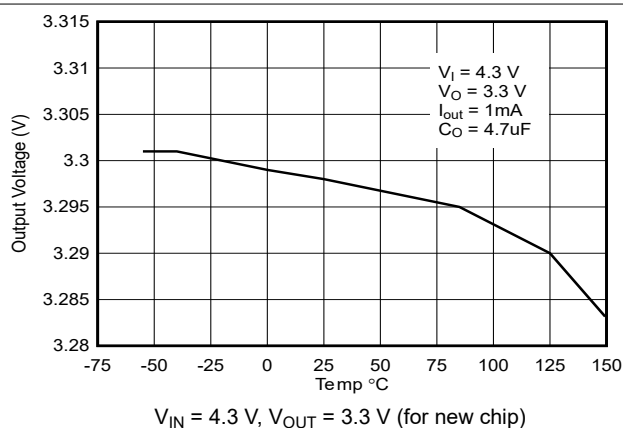
图 5-3. Output Voltage vs Temperature for New Chip
