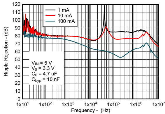
图 5-25. Ripple Rejection vs Frequency for New Chip
