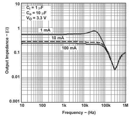
图 5-26. Output Impedance vs Frequency for Legacy Chip
