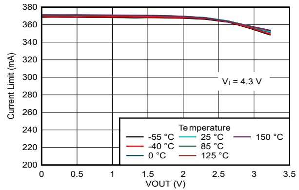
图 5-14. Short-Circuit Current vs Output Voltage for New Chip
