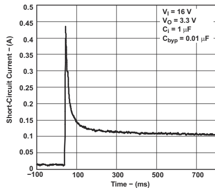
图 5-9. Short-Circuit Current vs Time for Legacy Chip
