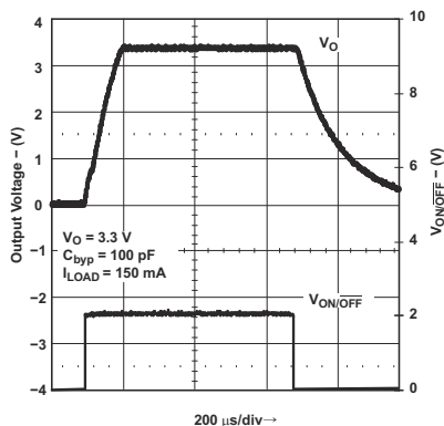
图 7-17. Turn-On Time for Legacy Chip
