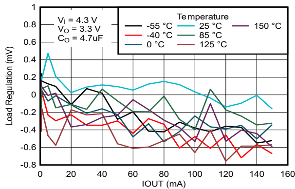
图 5-7. Output Regulation vs Load Current for New Chip
