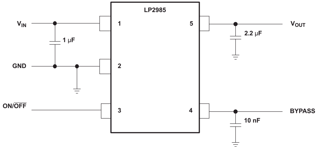
图 7-2. LP2985 Typical Application
