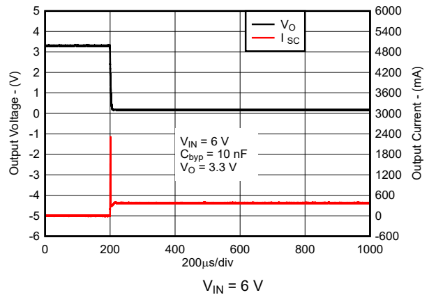
图 5-10. Short-Circuit Current vs Time for New Chip
