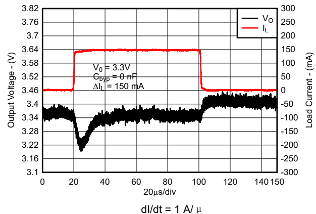
图 7-8. Load Transient Response for New Chip
