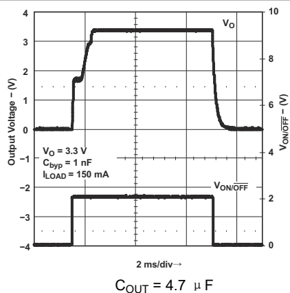
图 7-21. Turn-On Time for Legacy Chip
