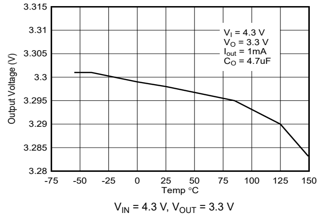
图 6-2. Output Voltage vs Temperature for New Chip
