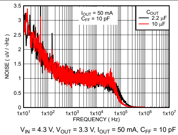
图 6-36. Output Noise Density vs C_{OUT} for New Chip
