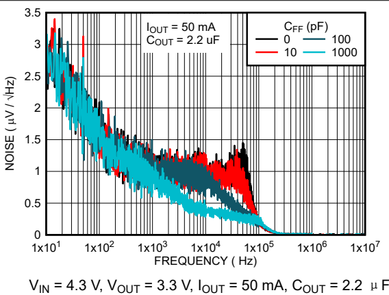
图 6-35. Output Noise Density vs C_{FF} for New Chip
