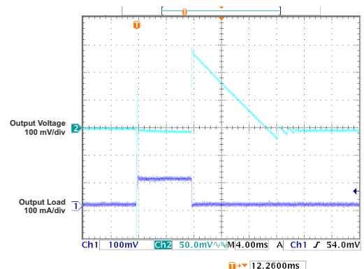
图 5-47. Load Transient Response vs Time ( V_{OUT} = 5\text{V} , C_L = 10\text{ }\mu\text{F} ) (Legacy Chip)
