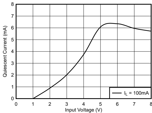
图 5-15. Quiescent Current vs Input Voltage ( I_L = 100\text{mA} )(Legacy Chip)
