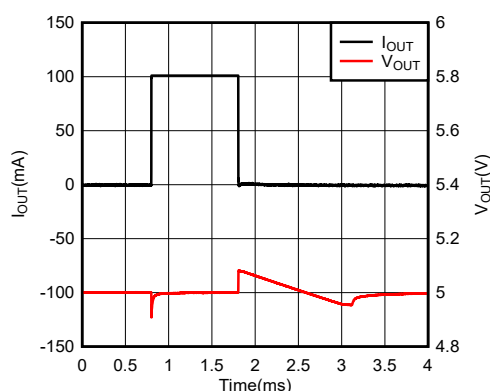
图 7-6. Load Transient Response vs Time (New Chip)
