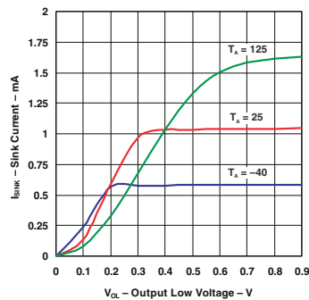
图 5-33. LP2951 \overline{\text{ERROR}} Comparator Sink Current vs Output Low Voltage (Legacy Chip)
