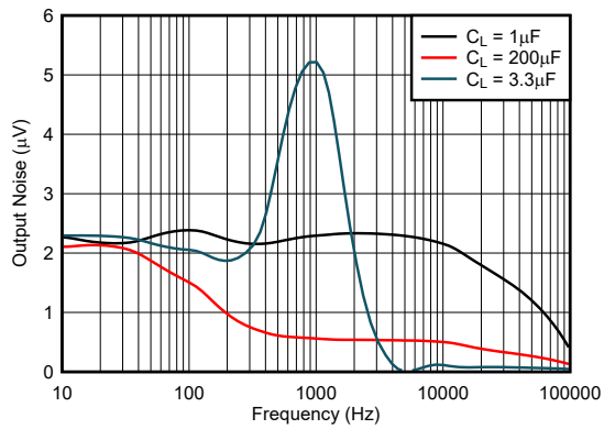
图 5-61. Output Noise vs Frequency (Legacy Chip)
