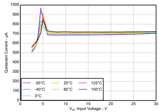
图 5-14. Quiescent Current vs Input Voltage ( I_L = 1\text{mA} )(New Chip)
