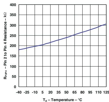
图 5-35. LP2951 Divider Resistance vs Temperature (Legacy Chip)
