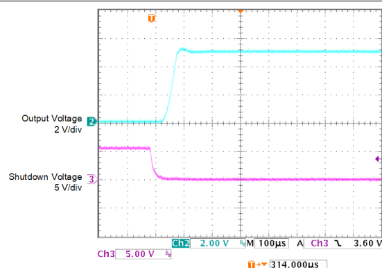
图 5-50. Enable Transient Response vs Time ( I_L = 1\text{mA} , C_L = 1\text{ }\mu\text{F} ) (Legacy Chip)
