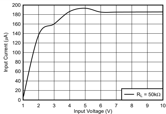
图 5-5. Input Current vs Input Voltage ( R_L = 50\text{k}\Omega )
