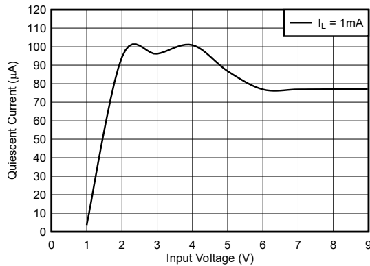
图 5-13. Quiescent Current vs Input Voltage ( I_L = 1\text{mA} )(Legacy Chip)
