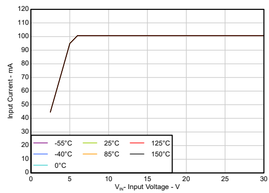
图 5-8. Input Current vs Input Voltage ( R_L = 50\text{ }\Omega ) (New Chip)
