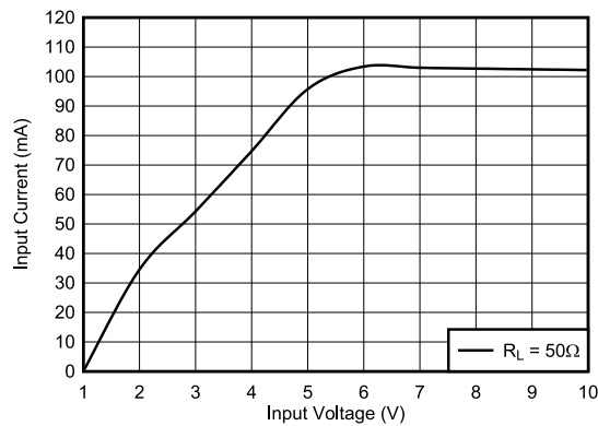
图 5-7. Input Current vs Input Voltage ( R_L = 50\text{ }\Omega ) (Legacy Chip)
