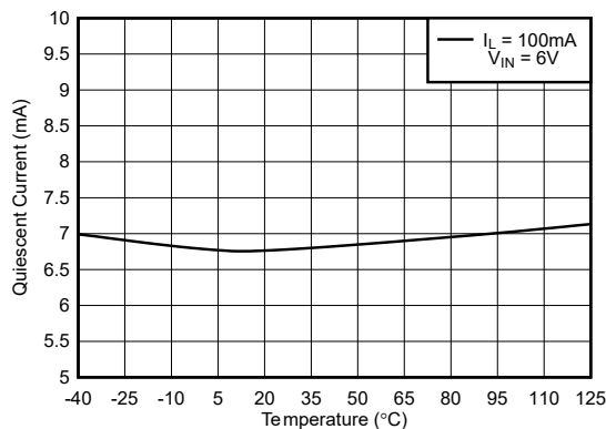
图 5-17. Quiescent Current vs Temperature ( I_L = 100\text{mA} )(Legacy Chip)
