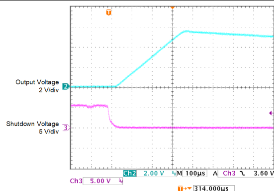
图 5-52. Enable Transient Response vs Time ( I_L = 1\text{mA} , C_L = 10\text{ }\mu\text{F} )
