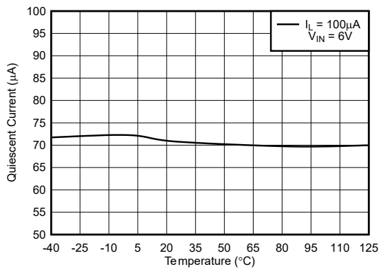
图 5-19. Quiescent Current vs Temperature ( I_L = 100\text{ }\mu\text{A} )(Legacy Chip)
