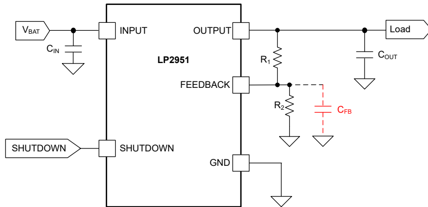
图 7-3. Formation of Parasitic Capacitor at the FB Pin
