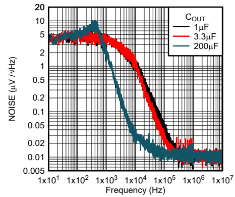
图 5-62. Output Noise vs Frequency (New Chip)
