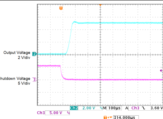
图 5-50. Enable Transient Response vs Time ( I_L = 1\text{mA} , C_L = 1\text{ }\mu\text{F} ) (Legacy Chip)
