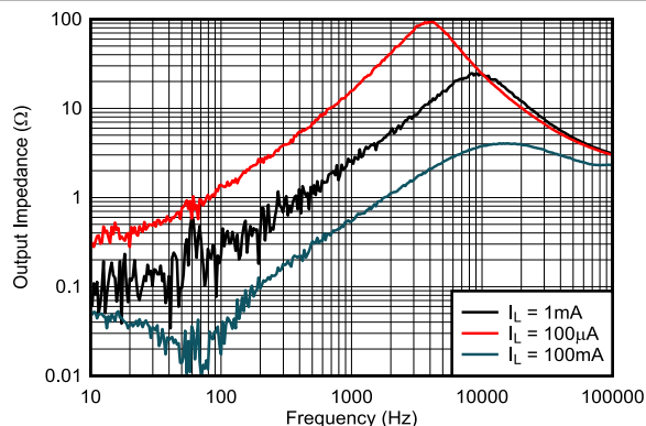
图 5-54. Output Impedance vs Frequency (Legacy Chip)
