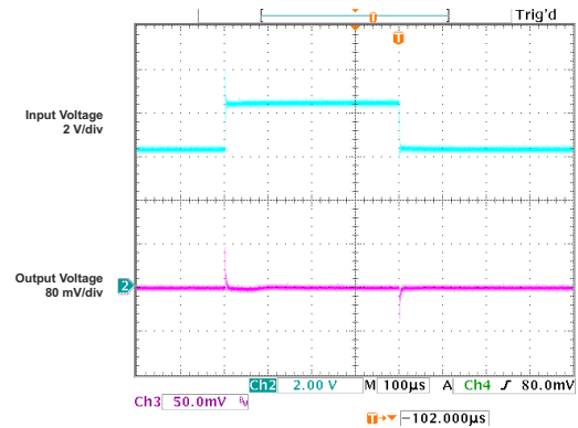
图 5-45. Line Transient Response vs Time (Legacy Chip)
