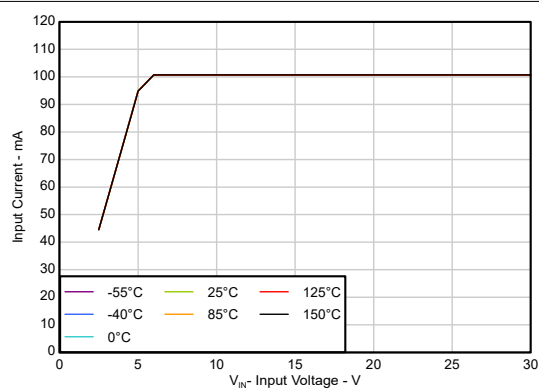
图 5-8. Input Current vs Input Voltage ( R_L = 50\text{ }\Omega ) (New Chip)
