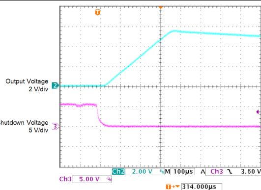
图 5-52. Enable Transient Response vs Time ( I_L = 1\text{mA} , C_L = 10\text{ }\mu\text{F} )
