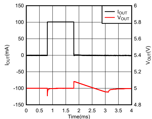
图 7-6. Load Transient Response vs Time (New Chip)
