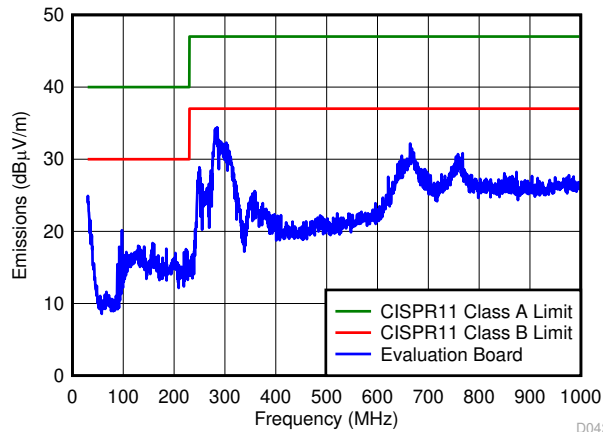
V_{IN} = 24\text{ V} I_{OUT} = 1\text{ A} Default EVM Layout with added 3 \times 100\text{pF} 0603 C_{IN}
