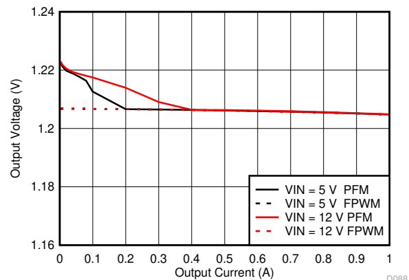
图 8-39. Line and Load Regulation for V_{OUT} = 1.2\text{ V}
