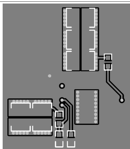
图 34. Typical Bottom-Layer Layout
