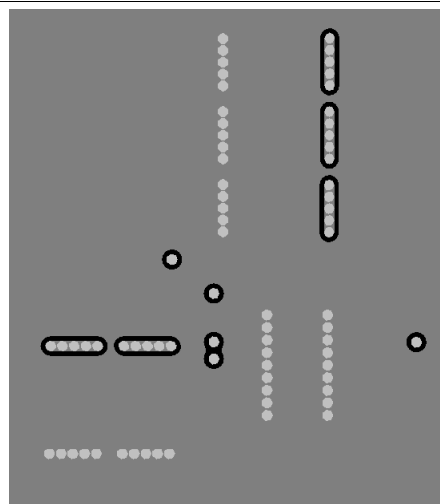
图 32. Typical Layer-2 Layout
