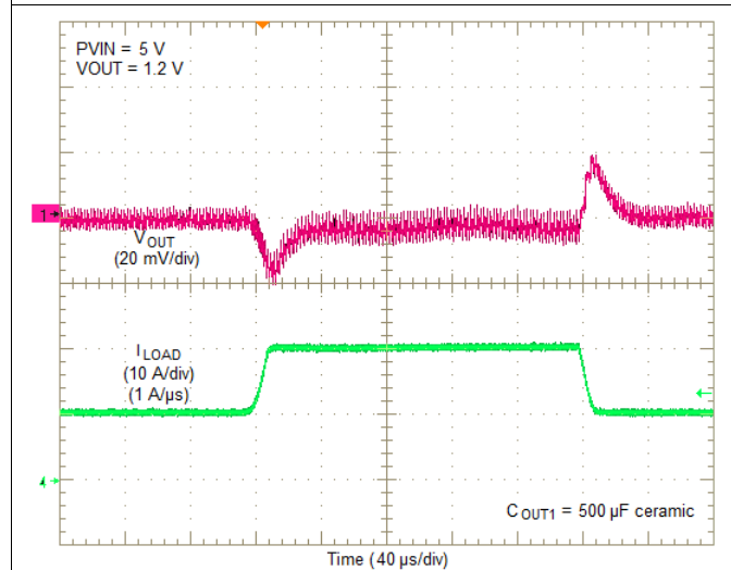
Figure 15. PV_{IN} = 5\text{V} , V_{OUT} = 1.2\text{V} , 10A Load Step
