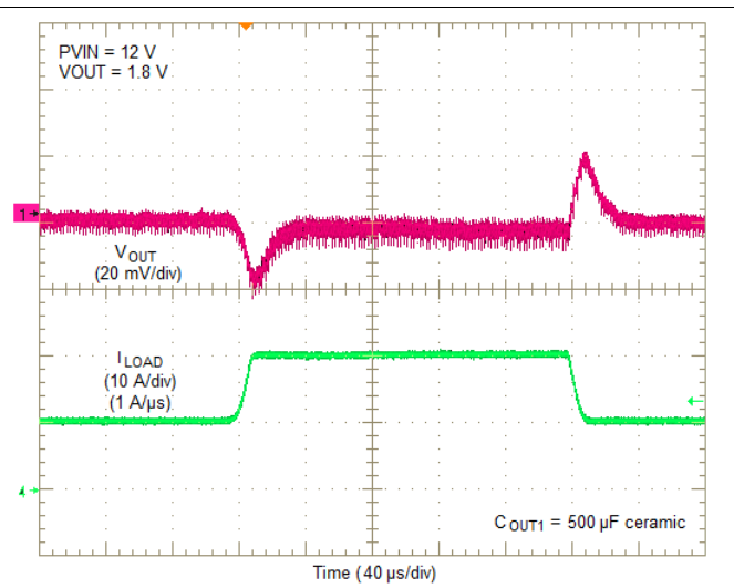
Figure 14. PV_{IN} = 12\text{V} , V_{OUT} = 1.8\text{V} , 10A Load Step
