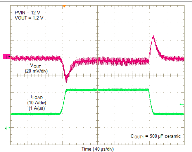
Figure 16. PV_{IN} = 12\text{V} , V_{OUT} = 1.2\text{V} , 5A Load Step
