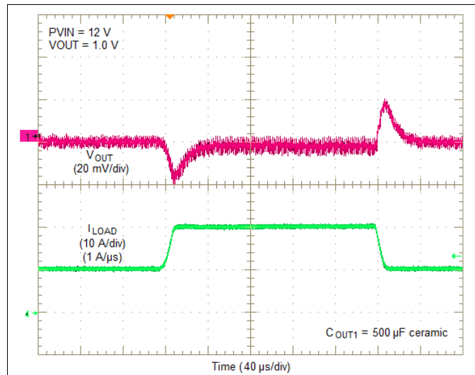
Figure 13. PV_{IN} = 12\text{V} , V_{OUT} = 1.0\text{V} , 10A Load Step
