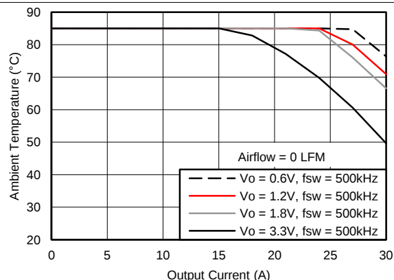
Figure 4. Safe Operating Area (0 LFM)
