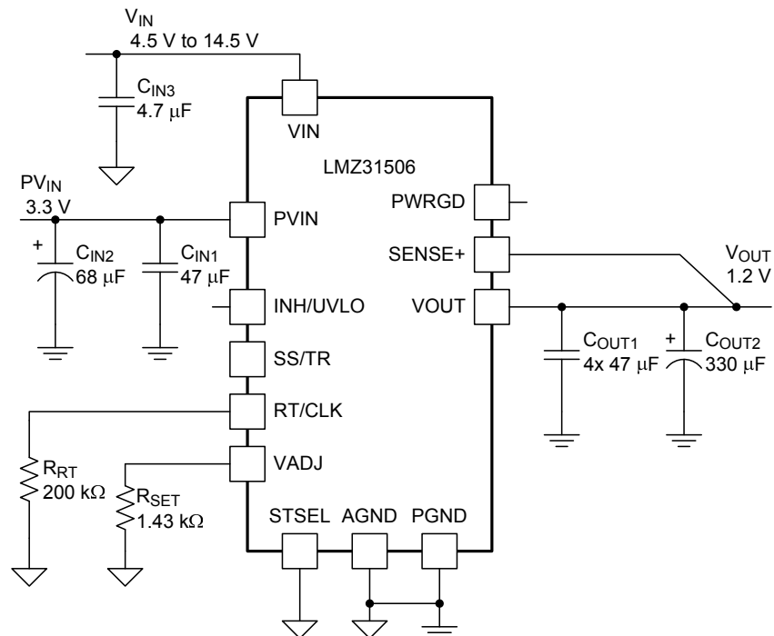
Figure 25. Typical Schematic P_{VIN} = 3.3 \text{ V} , V_{IN} = 4.5 \text{ V to } 14.5 \text{ V} , V_{OUT} = 1.2 \text{ V}
