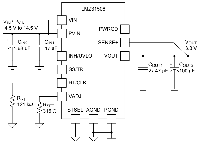
Figure 24. Typical Schematic P_{VIN} = V_{IN} = 4.5 \text{ V to } 14.5 \text{ V} , V_{OUT} = 3.3 \text{ V}
