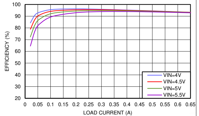
图 8-21. Efficiency V_{OUT} = 3.3\text{ V}
