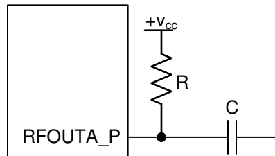
图 8-2. Resistor Pullup
