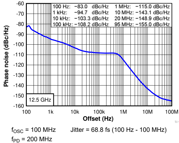
图 6-8. Closed Loop Phase Noise at 12.5 GHz
