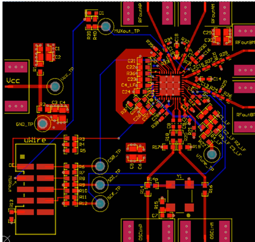
图 8-13. Recommended Layout
