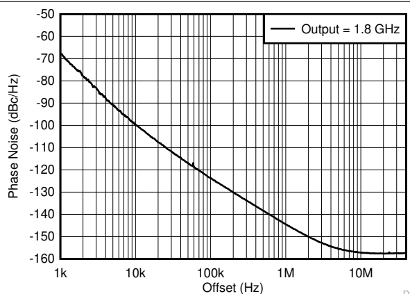
图 6-5. 1.8-GHz Output - Open-Loop Phase Noise
