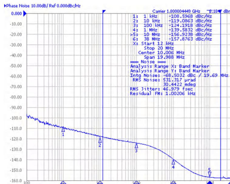
图 8-12. Typical Jitter
