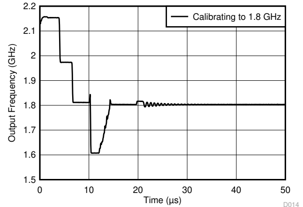
图 6-15. 20-μs Frequency Change Time to 1.8 GHz With Fast Calibration
