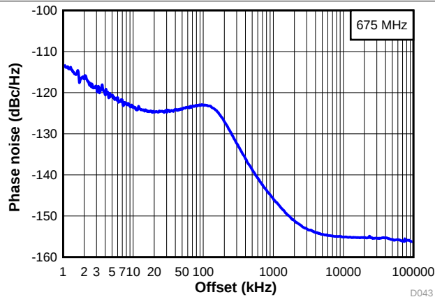
图 13. Wide Band Phase Noise at 675 MHz
