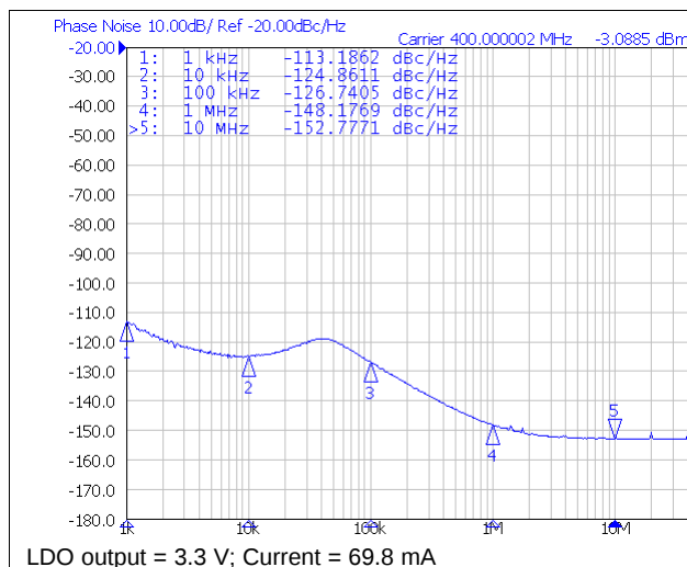
图 175. Phase Noise With LDO Power Supply
