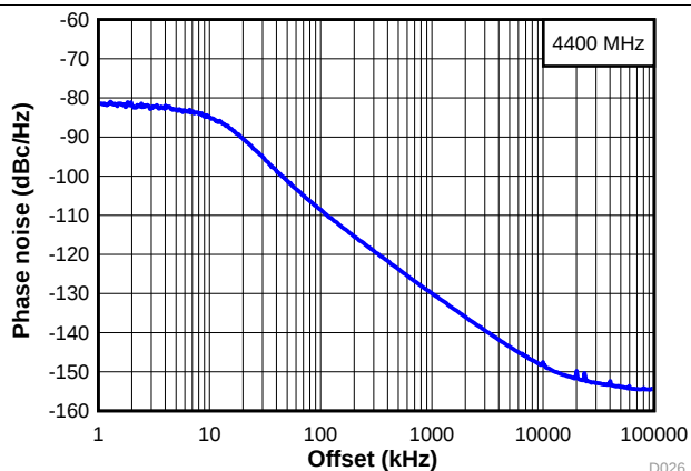
图 14. Narrow Band Phase Noise at 4.4 GHz
