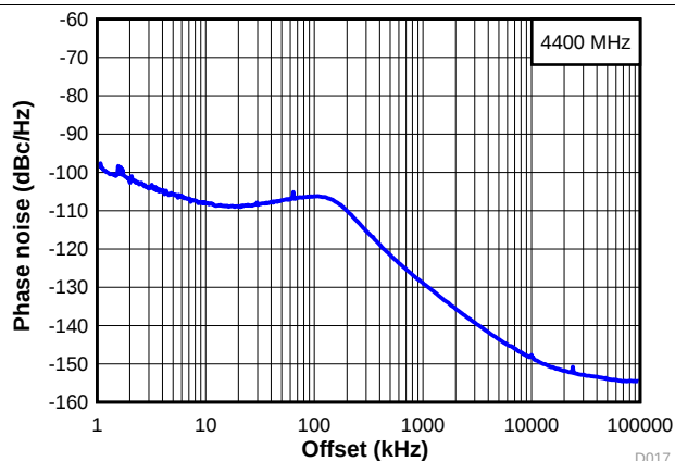
图 13. Wide Band Phase Noise at 4.4 GHz
