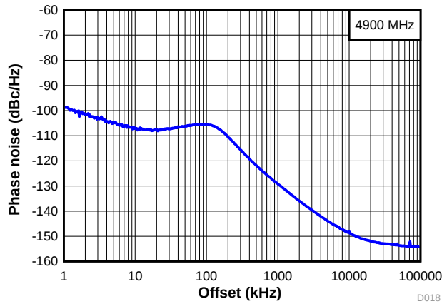
图 15. Wide Band Phase Noise at 4.9 GHz
