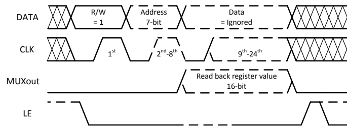
Figure 19. Register Readback Timing Diagram
