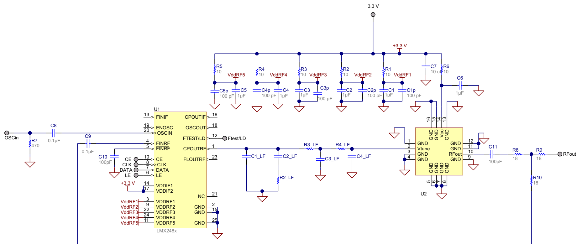
Figure 25. Typical Application
