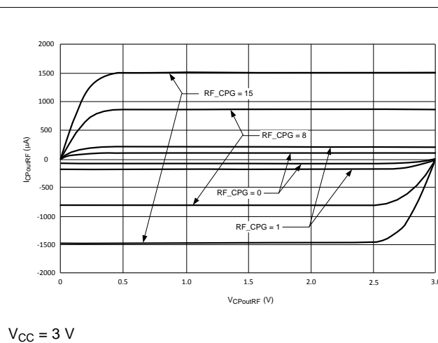
Figure 14. RF PLL Charge Pump Current
