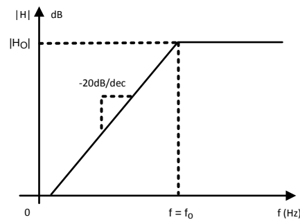
Figure 10. Highpass Filter Transfer Function
