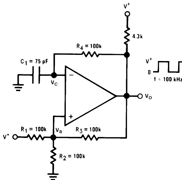
Figure 20. Squarewave Oscillator
