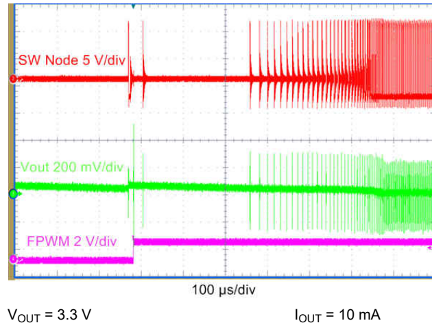
图 9-29. Mode Change Transient AUTO to FPWM mode
