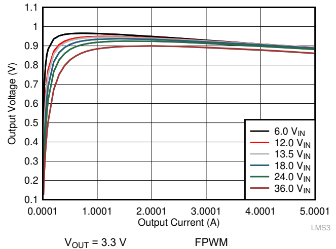
图 9-18. Efficiency
