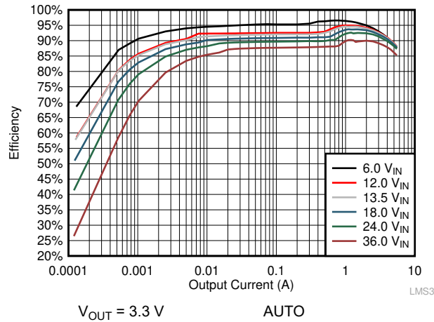
图 9-17. Efficiency
