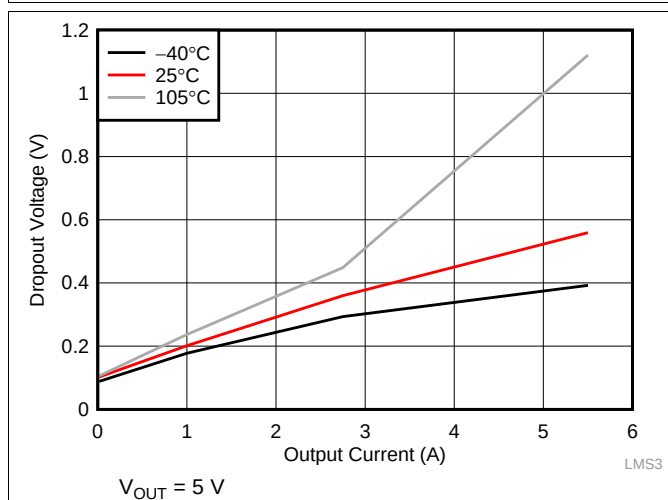
Figure 30. Dropout for \geq 330\text{ kHz}
