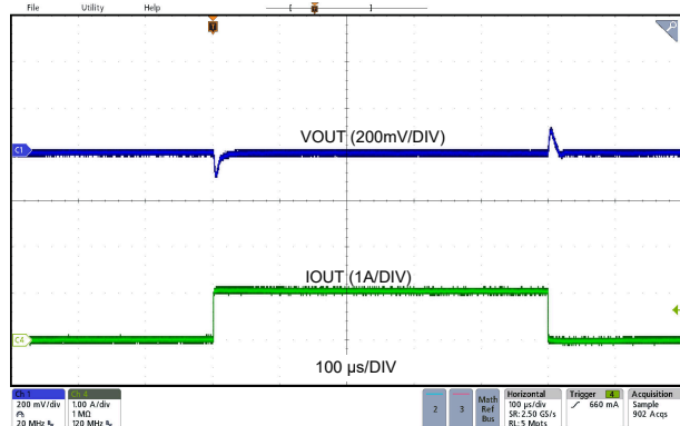
LMR66430MC3 V_{OUT} = 3.3V 2.2MHz (FPWM) 修复 0A 至 1A, 1A/µs
