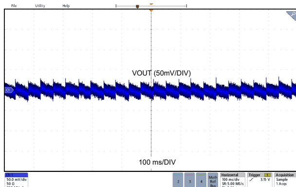
LMR66430MC3 V_{OUT} = 3.3V 空载 修复
