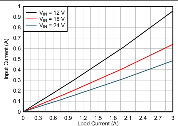
LMR66430MC3 V_{OUT} = 3.3V 2.2MHz (自动) 修复
