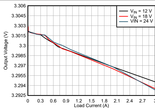
LMR66430MC3 V_{OUT} = 3.3V 2.2MHz (自动) 修复
