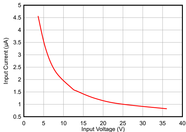
LMR66430MC3 V_{OUT} = 3.3V 2.2MHz (自动) 修复 空载
