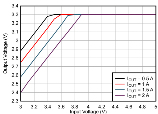
LMR66430MC3 V_{OUT} = 3.3V 2.2MHz (自动) 修复
