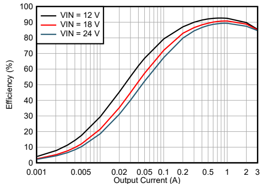
LMR66430MC3 V_{OUT} = 3.3V 2.2MHz (FPWM) 修复
