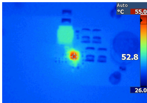
LMR66430MC3 V_{OUT} = 3.3V 12V_{IN} , 2A, 2.2MHz 修复
