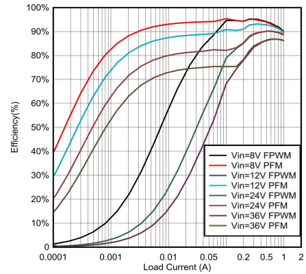
图 6-4. 5-V Efficiency Versus Load Current
