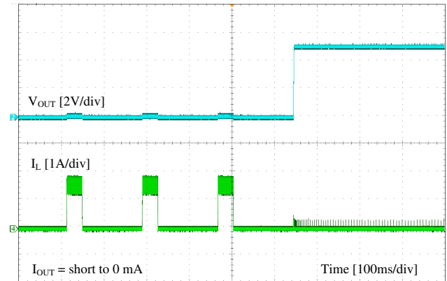
图 8-10. Short Recovery
