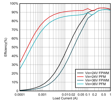
图 6-6. 12-V Efficiency Versus Load Current
