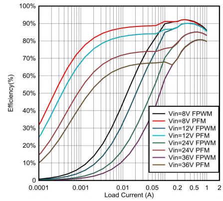
图 6-2. 3.3-V Efficiency Versus Load Current
