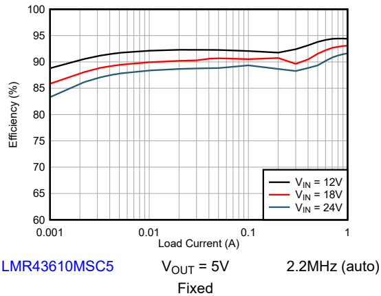
图 8-5. Efficiency
