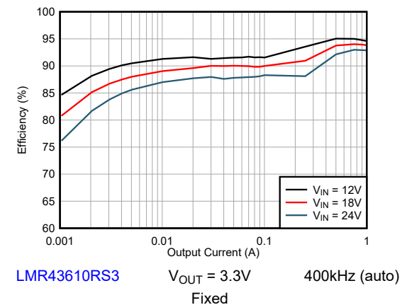
图 8-8. Efficiency
