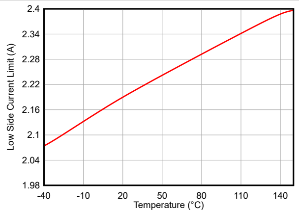
图 7-6. Low Side MOSFET Current Limit Versus Temperature
