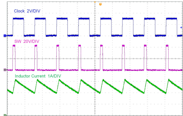
LMR38025-Q1 V_{OUT} = 5V 400kHz 2μs/DIV
