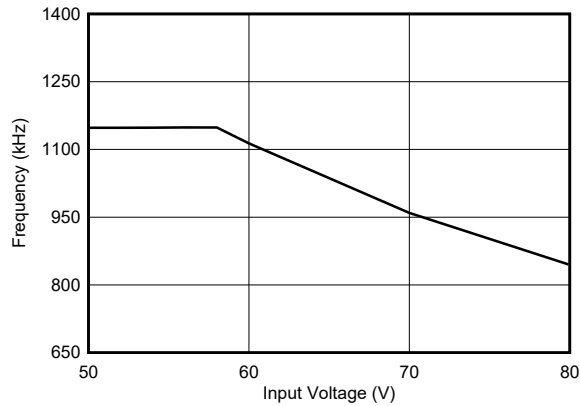
F_{SW} = 1.1 \text{ MHz} V_{OUT} = 5 \text{ V} I_{OUT} = 1 \text{ A} 图 7-8. Typical Frequency Foldback at T_{ON\_MIN}
