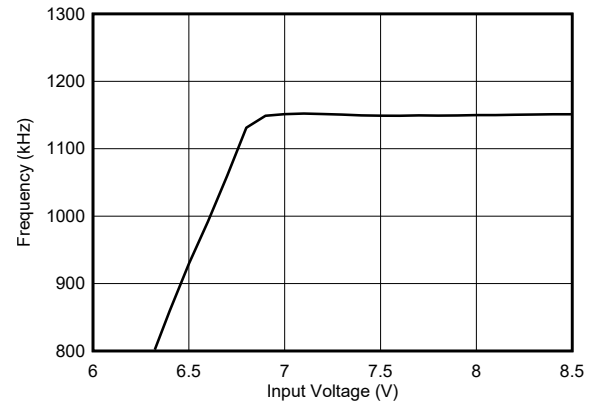
F_{SW} = 1.1 \text{ MHz} V_{OUT} = 5 \text{ V} I_{OUT} = 1 \text{ A} 图 7-9. Typical Frequency Foldback at T_{OFF\_MIN}
