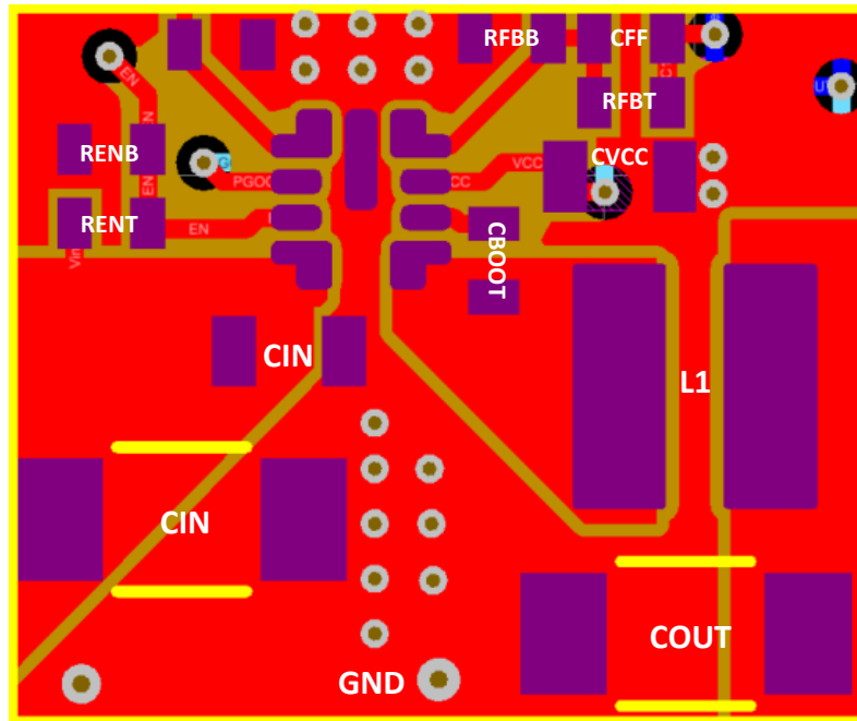
Figure 9-20. Example Layout
