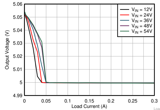
LMR36503R5 V_{OUT} = 5V Fixed 400 kHz (AUTO)
