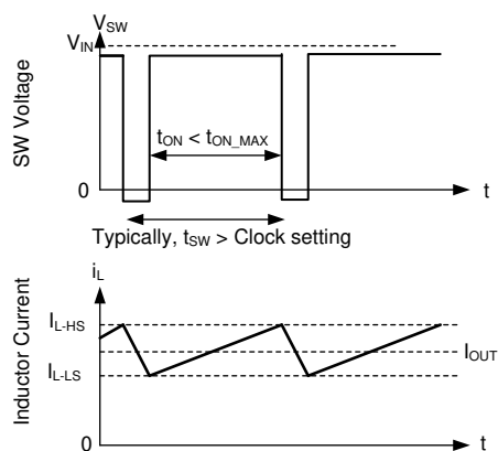
图 8-10. Current Limit Waveforms
