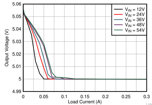
LMR36503R5 V_{OUT} = 5V Fixed 1 MHz (AUTO)
