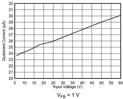
图 8-1. Non-Switching Input Supply Current
