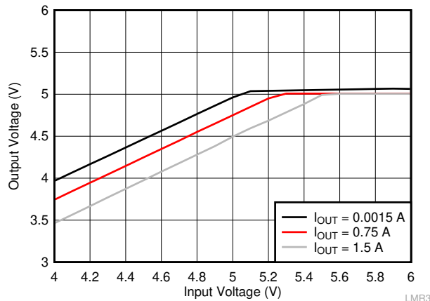
图 9-9. Overall Dropout Characteristic V_{OUT} = 5\text{ V}
