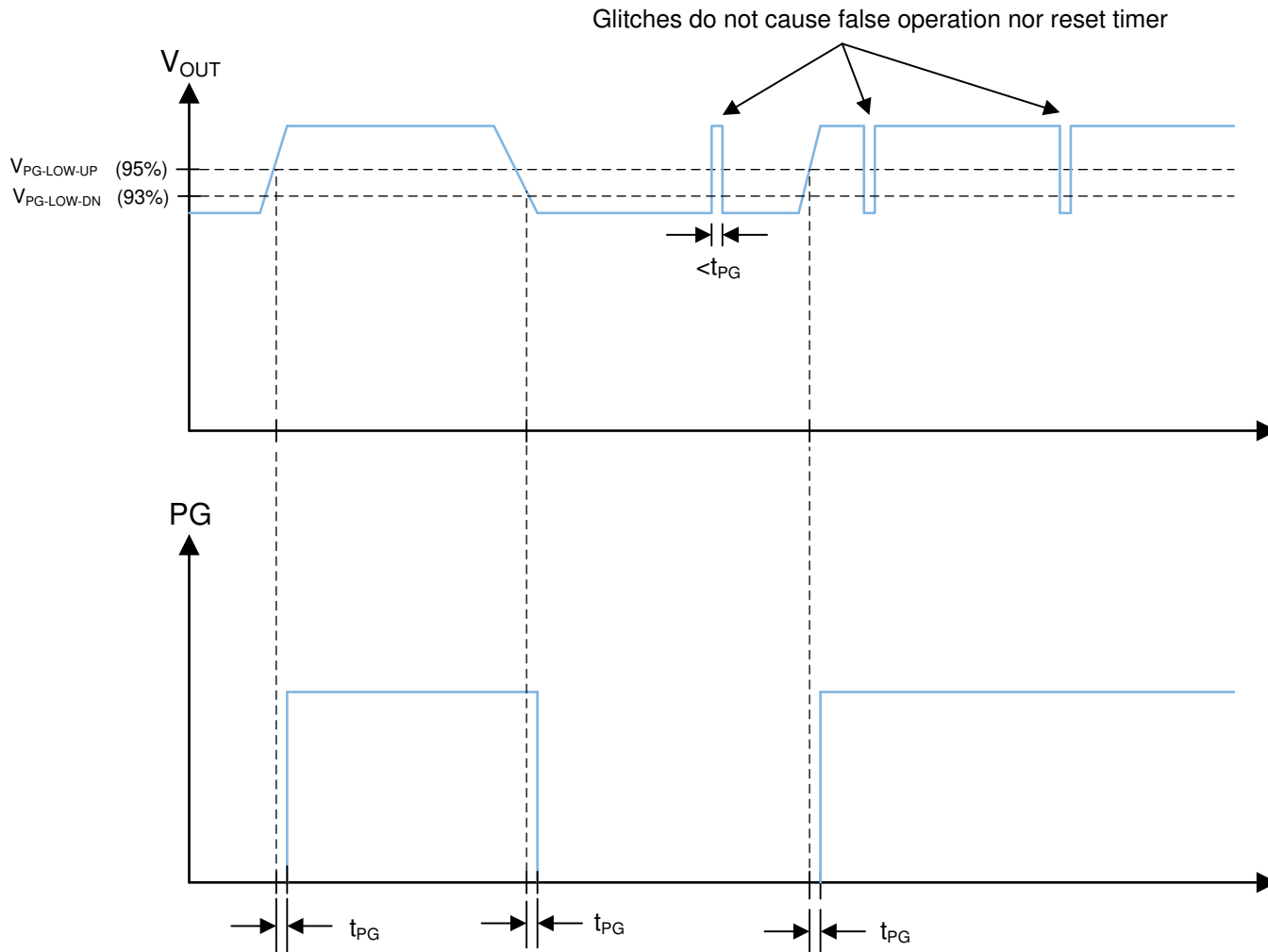
图 9. Power-Good-Timing Behavior
