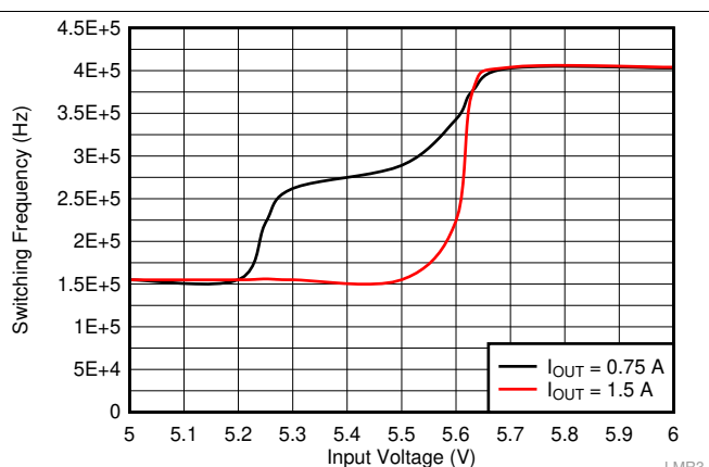
图 16. Frequency Dropout Characteristics f_{sw} = 400\text{ kHz}
