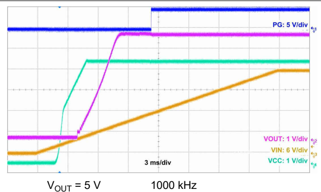
图 10-33. Start-Up Waveform
