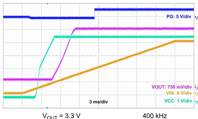
图 10-15. Start-Up Waveform
