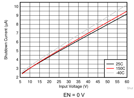
图 8-2. Shutdown Supply Current
