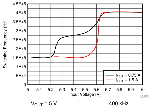
图 10-11. Frequency Dropout Characteristic
