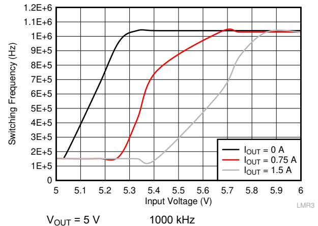
图 10-31. Frequency Dropout Characteristic
