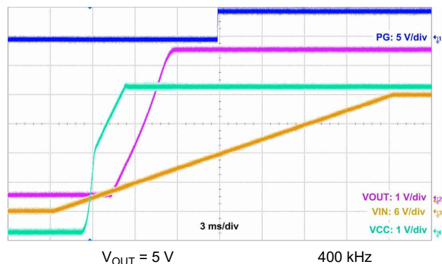
图 10-14. Start-Up Waveform
