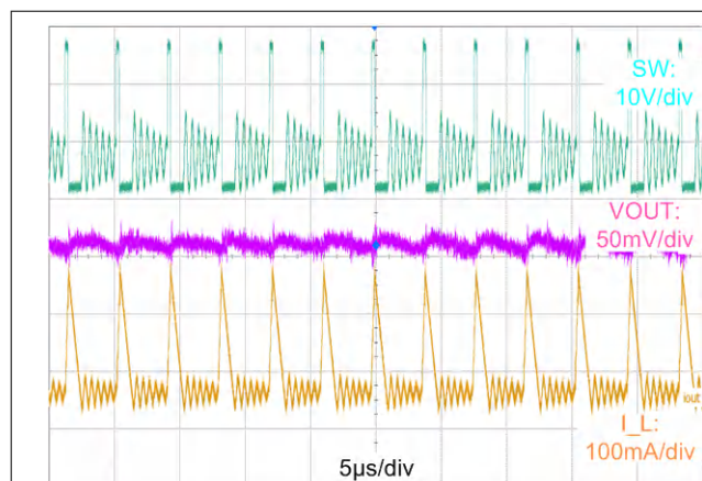
图 8-7. Typical PFM Switching Waveforms V_{IN} = 24 V, V_{OUT} = 5 V, I_{OUT} = 30 mA
