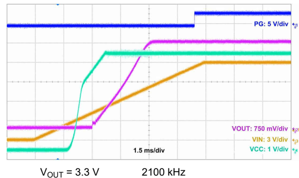
图 9-31. Start-Up Waveform
