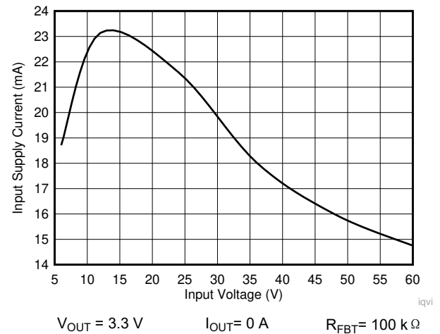
图 9-30. Input Supply Current
