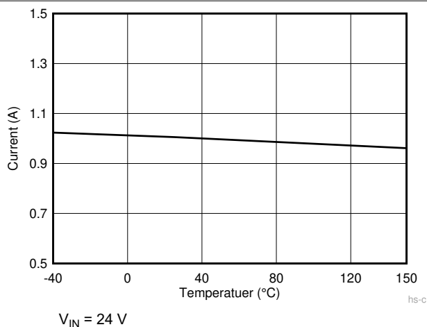
图 7-3. High Side Current Limit
