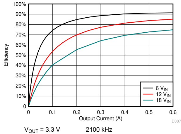
图 9-27. Efficiency
