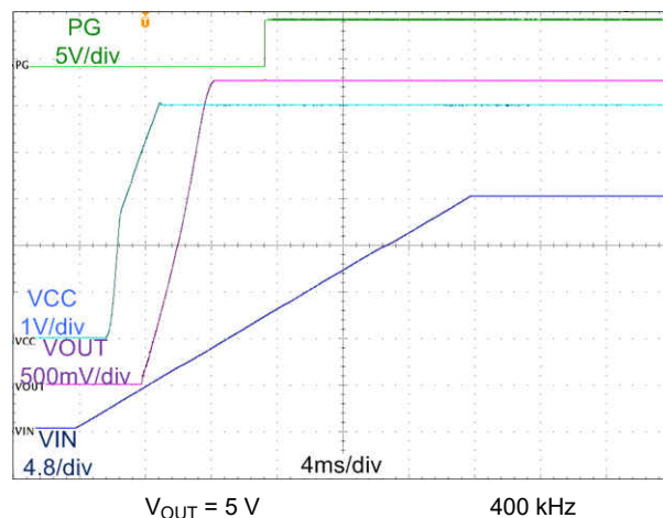
图 9-14. Start-Up Waveform
