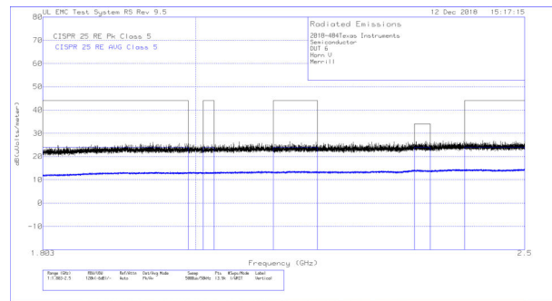
图 9-24. Radiated EMI Horn Vertical vs. CISPR25 Limits
