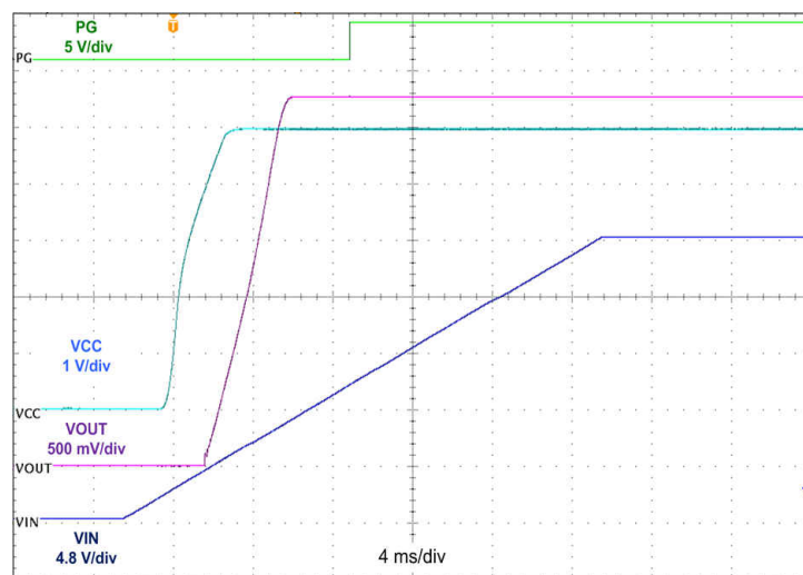
图 8-5. Typical Start-up Behavior V_{IN} = 24\text{ V} , V_{OUT} = 3.3\text{ V} , I_{OUT} = 0.6\text{ A}
