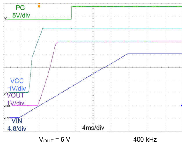
图 9-13. Start-Up Waveform
