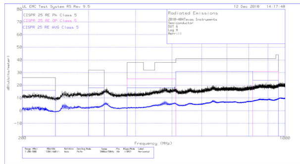
图 9-23. Radiated EMI Log Horizontal vs. CISPR25 Limits
