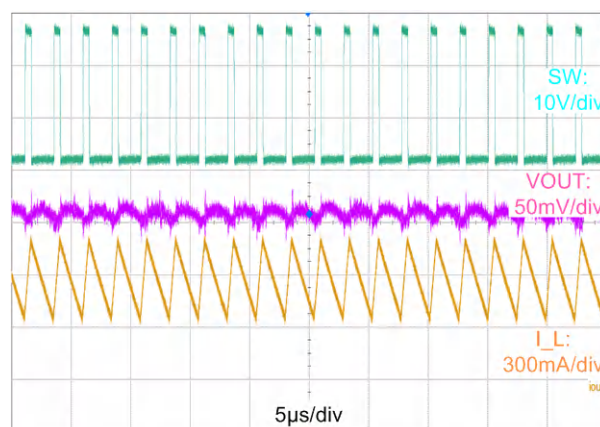
图 8-8. Typical PWM Switching Waveforms V_{IN} = 24 V, V_{OUT} = 5 V, I_{OUT} = 600 mA, f_s = 400 kHz
