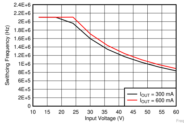
图 9-29. Switching Frequency vs Input Voltage
